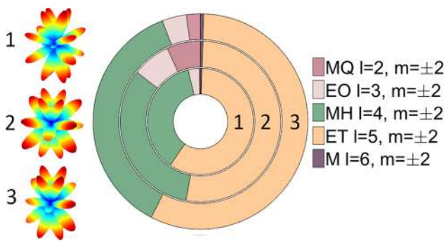
Figure 7: Comparison of the far-field diagrams and multipolar compositions of the SHG electromagnetic field and the disk's eigenmode at the SH frequency for parameters of the maximum SHG efficiency ( \lambda_0=1600 nm, r=470 nm, h=645 nm): 1 - SH mode, 2 - AP beam excitation, 3 - PW excitation. E/M-electric/magnetic multipoles, Q-quadrupole, O-octupole, H-hexadecapole, T-triacontadipole
