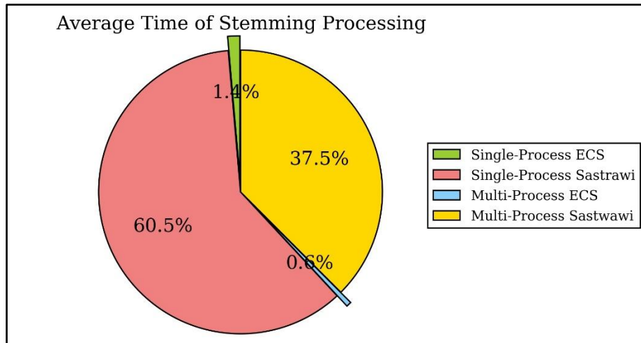
Fig 4: Results comparison for average time of stemming processing
