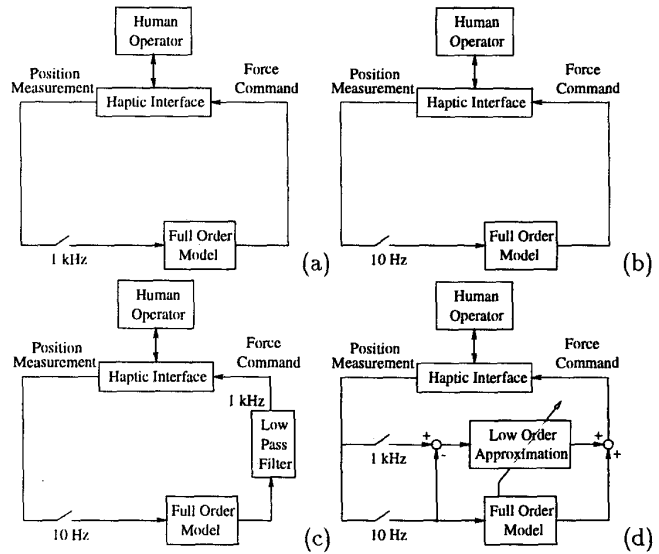
Figure 1: Simulation paradigms.
