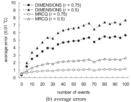
Fig. 12. Comparison of MRCQ and DIMENSIONS under different numbers of events.
