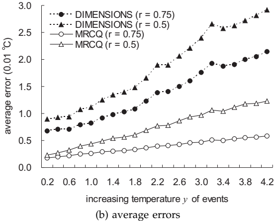
Fig. 11. Comparison of MRCQ and DIMENSIONS under different increasing temperatures of events.
