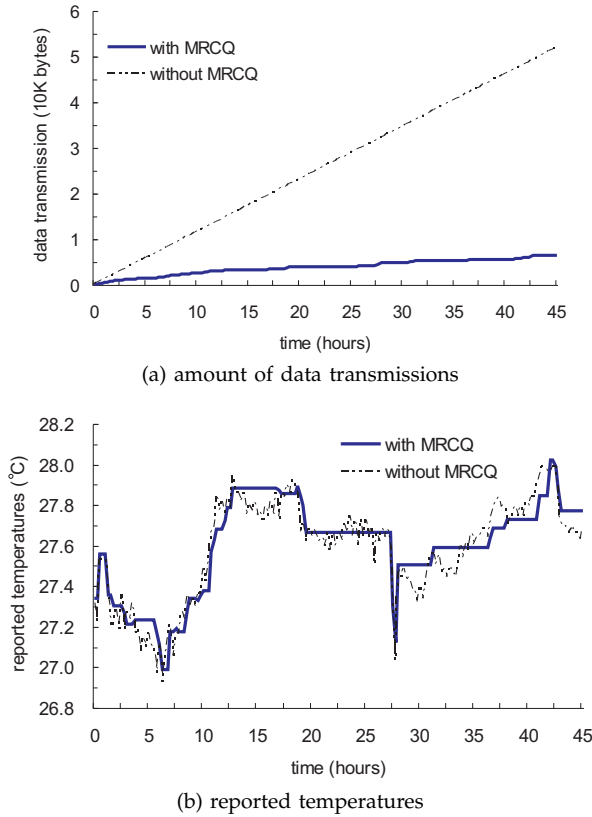
Fig. 8. Experimental results from the prototyping system.
