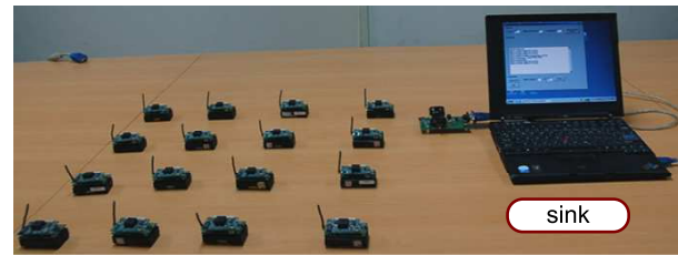
Fig. 7. A 16-mote prototype in our experiment.
