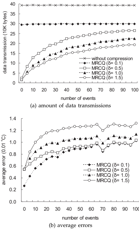
Fig. 15. Effect of the temporal compression algorithm.
