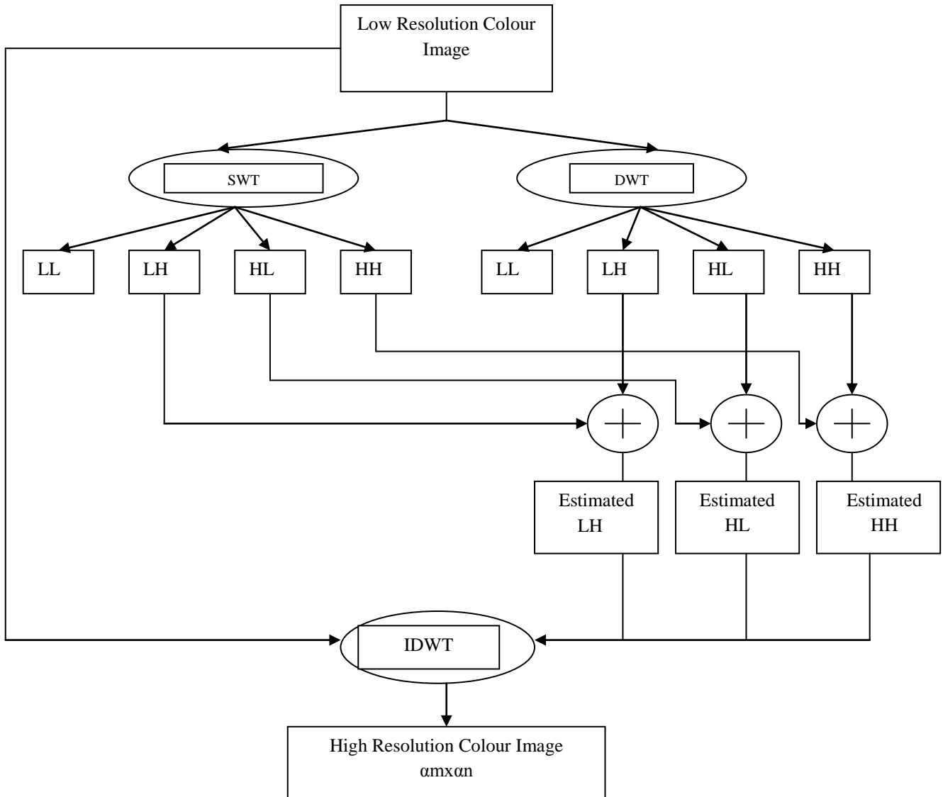
Fig.3 Block Diagram DWT and SWT based Image Resolution Enhancement
