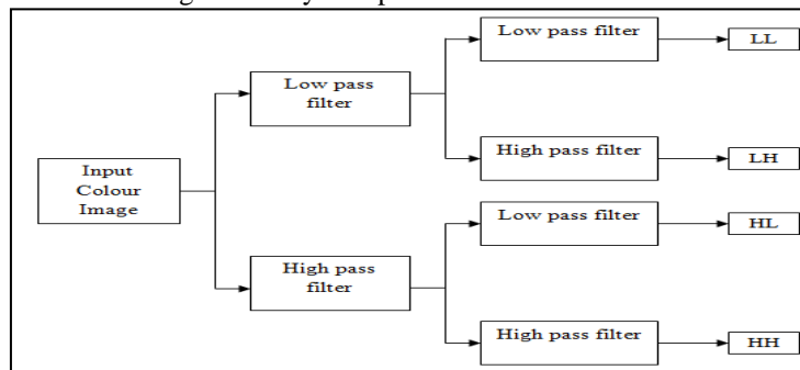
Fig.2 Block diagram of SWT Filter Banks of level.1
