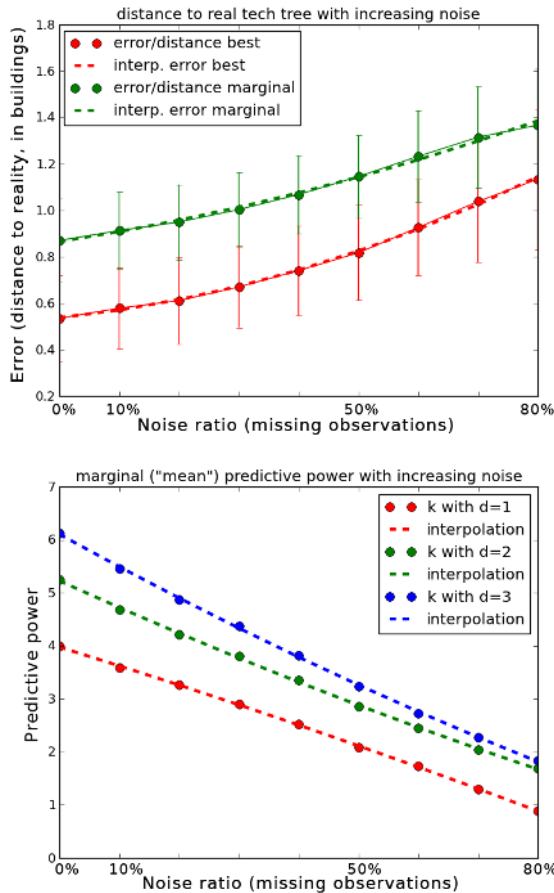
Fig. 7: Evolution of our metrics with increasing noise, from 0 to 80%. The top graphic shows the increase in distance between the predicted build tree, both most probable (“best”) and marginal (“mean”) and the actual one. The bottom graphic shows the decrease in predictive power: numbers of buildings ahead ( k ) for which our model predict a build tree closer than a fixed distance/error ( d ).
