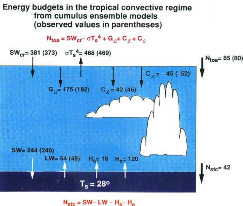
Figure 1. Energy fluxes at the top of the atmosphere and at the ocean-atmosphere interface as computed by the Goddard Cumulus Ensemble (GCE) model. Also included in parentheses are top-of-the-atmosphere fluxes estimated from the Earth Radiation Budget Experiment and surface flux estimates from radiation model for April 1985. The observed values (in parentheses) are averaged over the region from 100 to 180°E, 20°N to 20°S. Subscript “toa” denotes top of the atmosphere, subscript “cr” denotes clear-sky conditions, and subscript “sfc” denotes the surface. SW_{\text{cr}} is the net absorbed solar radiation averaged over the clear-sky region. T_s^4 is the longwave radiation emitted by the ocean surface. SW and LW stand for shortwave and longwave radiative heating/cooling, respectively. H_s and H_e stand for surface sensitive and latent heat fluxes, respectively. G_a is the atmospheric greenhouse effect. C_s and C_l are the longwave and shortwave cloud forcing, respectively. Units are in \text{W m}^{-2} . T_s is the ocean surface temperature. A reasonable agreement between the modeled and satellite observed budget is found. Adapted from Lau et al. [1994].
