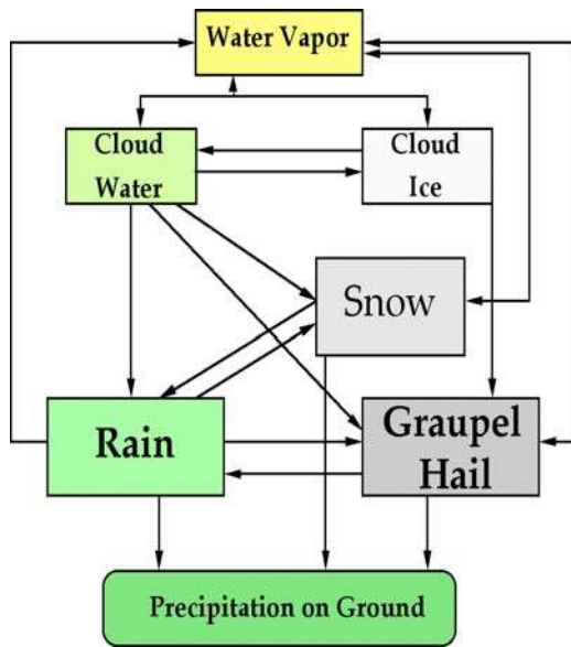
Figure 4. Representation of the three-class ice scheme used in the cloud model. Adapted from Tao and Moncrieff [2003].
