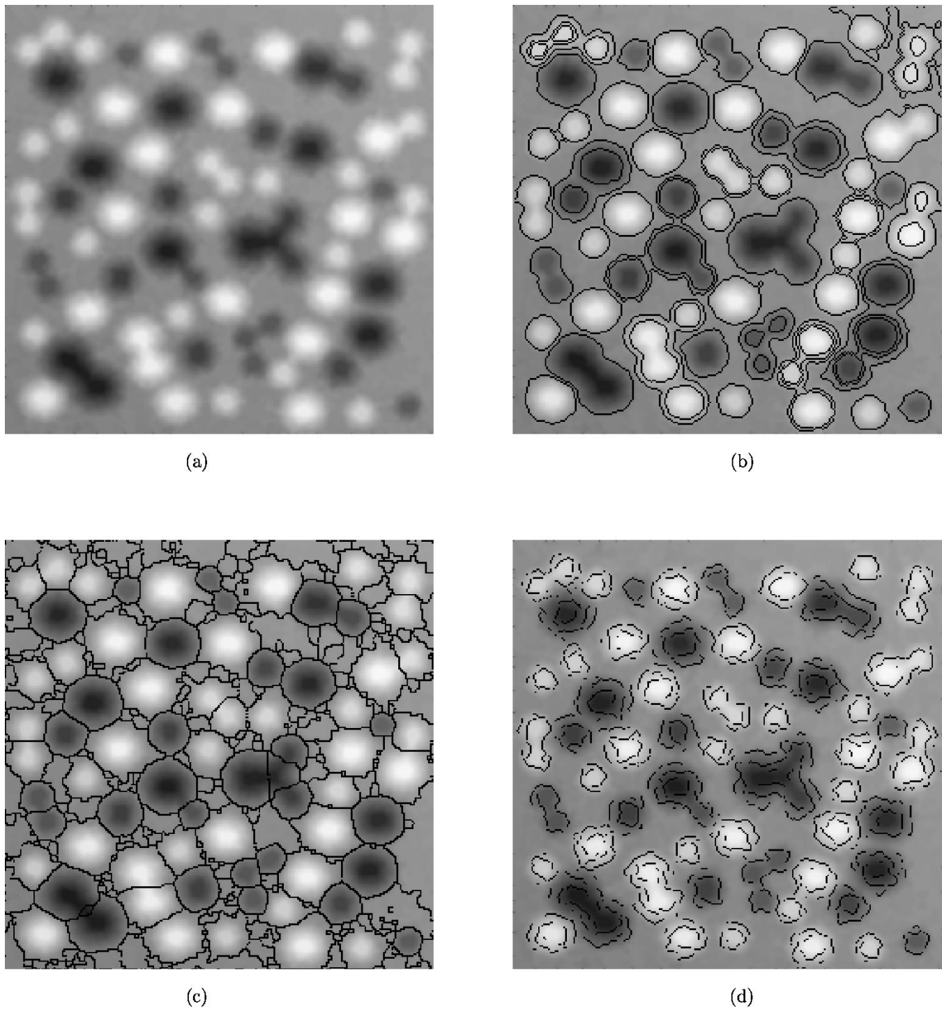
Fig. 8. Results of segmentation (a) (input image) noise-corrupted version of the image in Fig. 7(a) (b)–(d) output images, (b) multiscale morphological segmentation, (c) watershed segmentation, and (d) Canny's edge-based technique.
