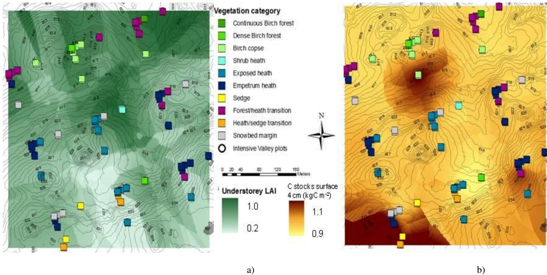
Figure 3.10: Kriged maps of the understorey LAI (a) and surface 4 cm C stocks (kg C m -2 ) (b)
