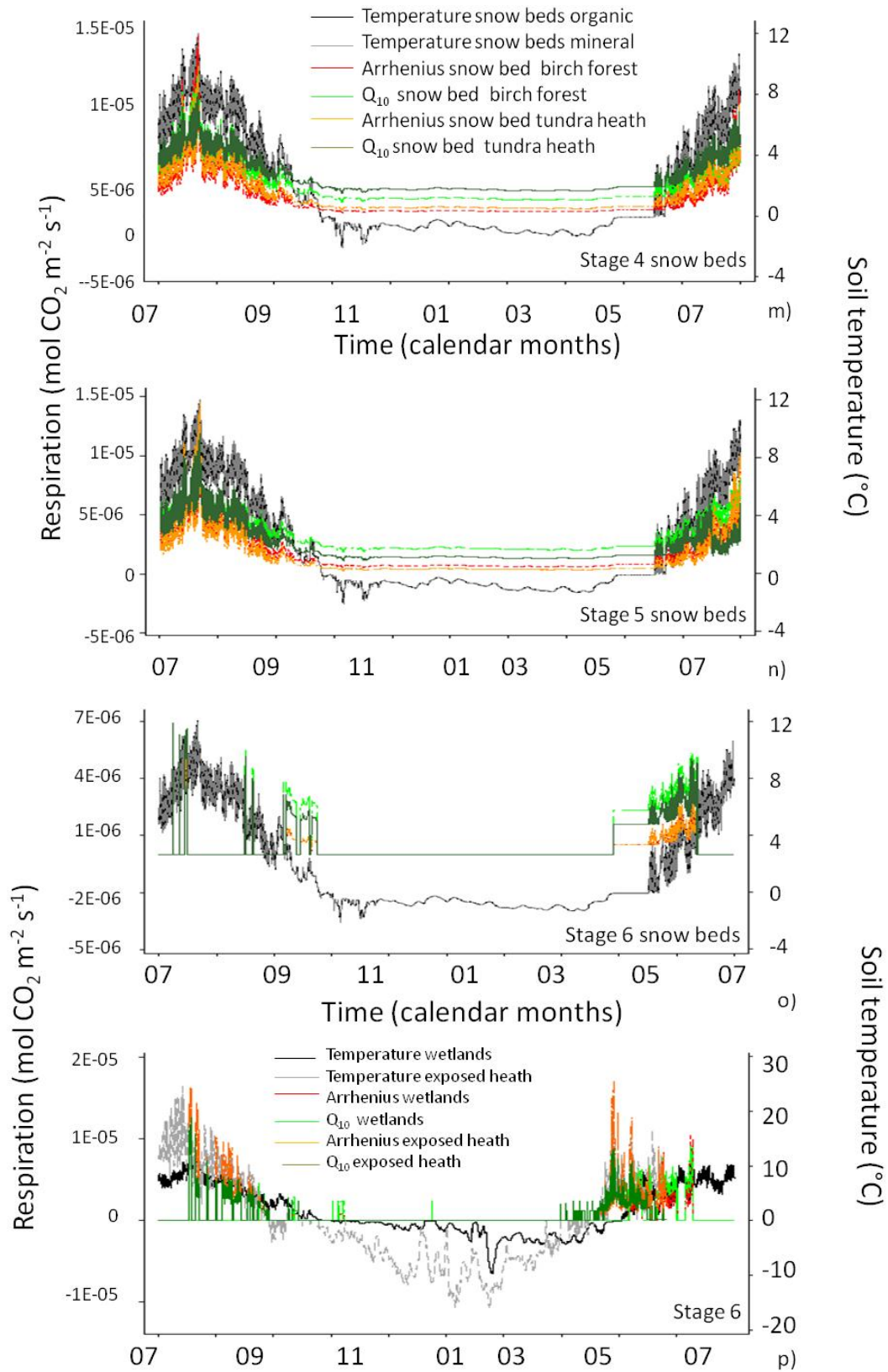
Figure 4.7: Soil respiration (mol CO 2 m -2 s -1 ) estimated with the Arrhenius and Q 10 equations for the snow beds profiles (Stage 4, m, 5, n, 6, o), Exposed heath and Sedge and wetlands soils (Stage 6, p) and associated temperature series (°C)
