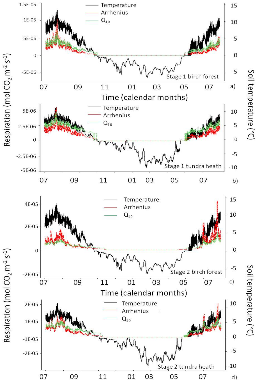
Figure 4.7: Soil respiration (mol CO 2 m -2 s -1 ) estimated with the Arrhenius and Q 10 equations for the birch forest (Stage 1, a), tundra heath (Stage 1, b), birch forest IV profile (Stage 2, c) and tundra heath IV profile (Stage 2, d) and associated temperature series (°C)
