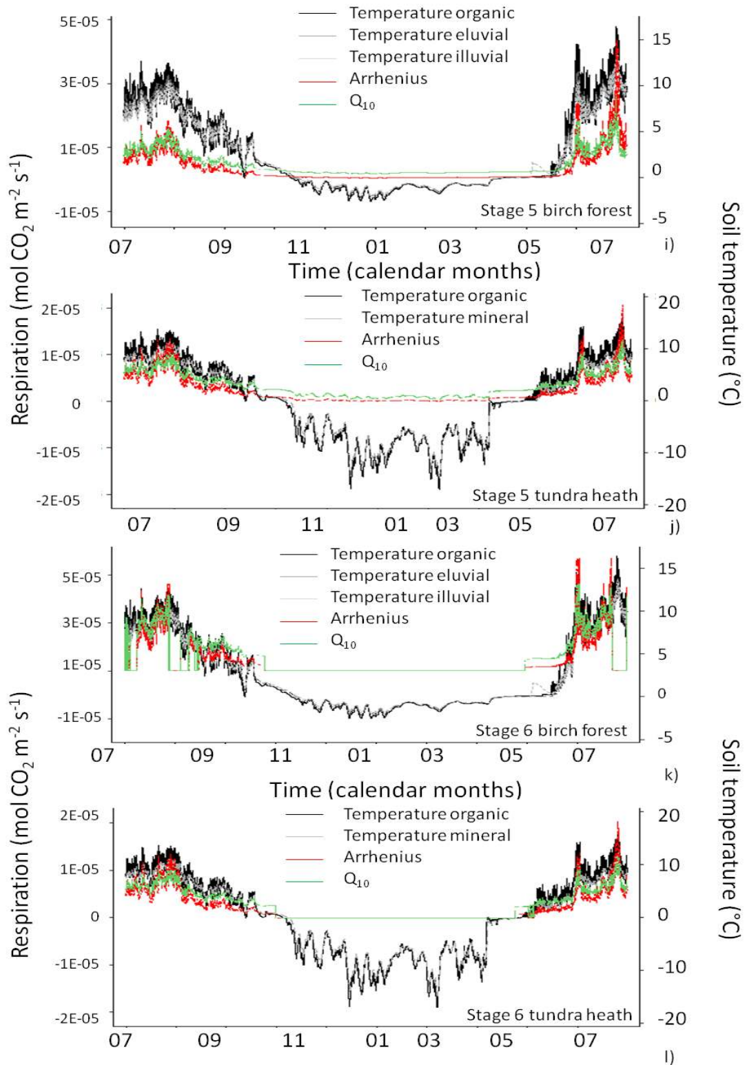
Figure 4.7: Soil respiration (mol CO 2 m -2 s -1 ) estimated with the Arrhenius and Q 10 equations for the birch forest IV profile (Stage 5, i, 6, k) and tundra heath IV profile (Stage 5, j, 6, l) and associated temperature series (°C)
