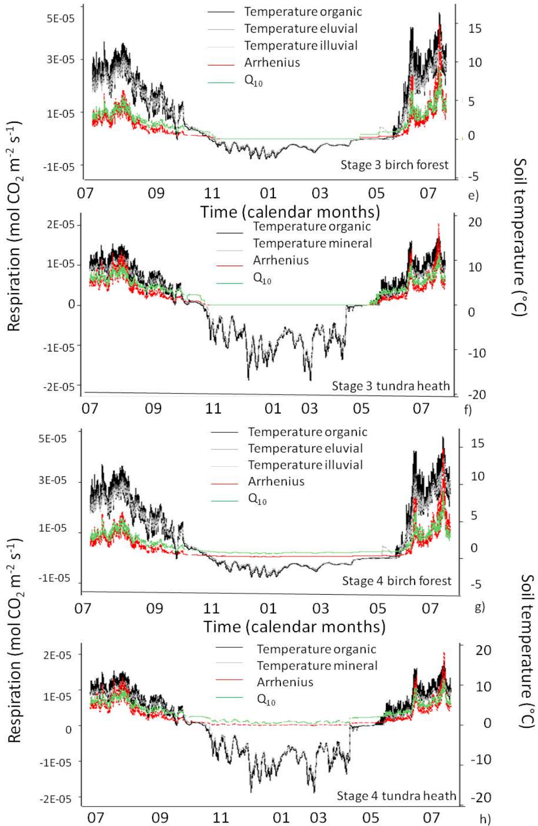
Figure 4.7: Soil respiration (mol CO 2 m -2 s -1 ) estimated with the Arrhenius and Q 10 equations for the birch forest IV profile (Stage 3, e, 4, g) and tundra heath IV profile (Stage 3, f, 4, h) and associated temperature series (°C)
