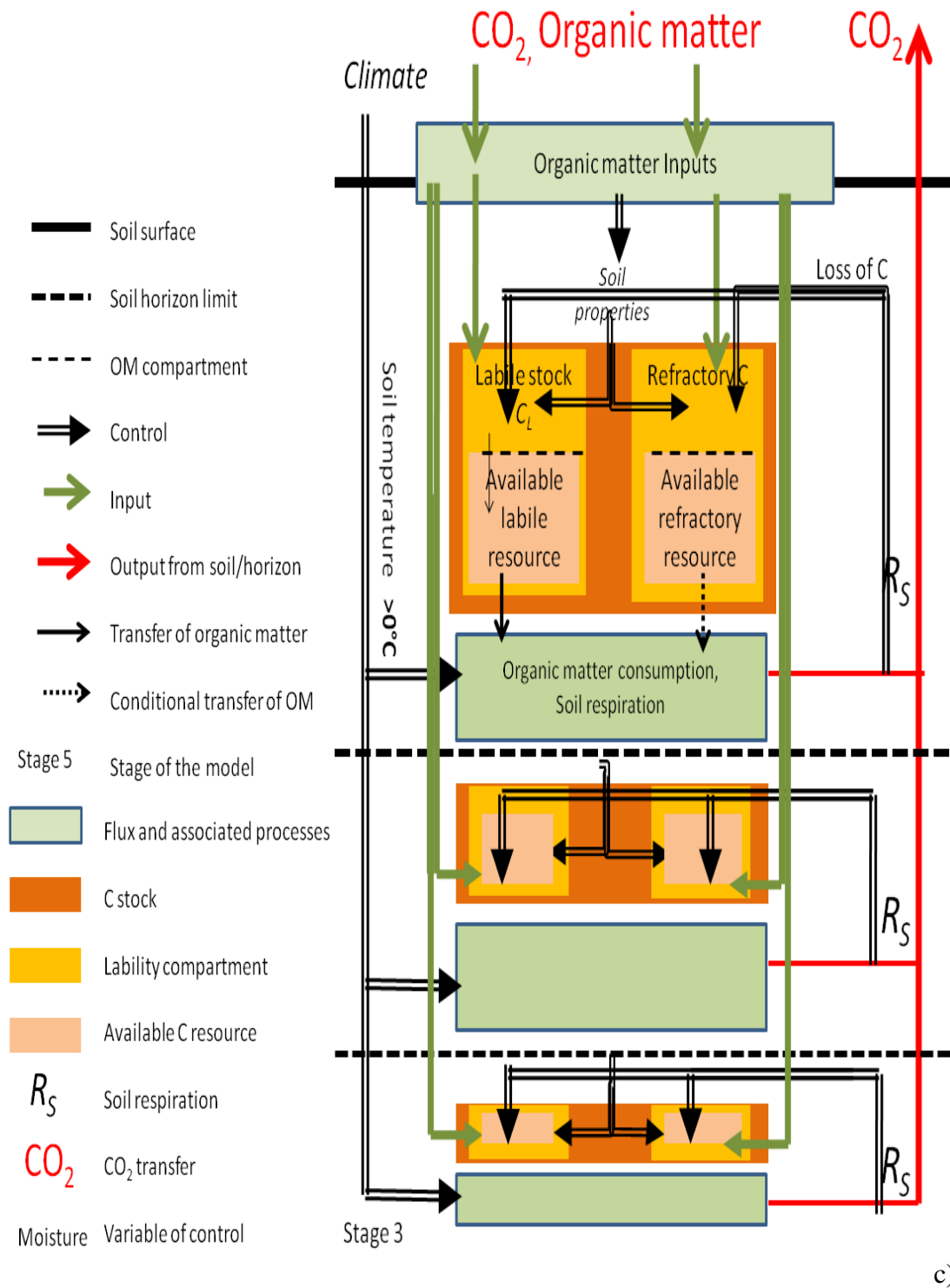
Figure 4.2 c: Stage 3 structure with several soil horizons; the inputs of CO_2 and organic matter going into the soil and ending up either in the labile or recalcitrant C compartment; the respiration rate is only function of the temperature and can use the stocks of labile C; variables are explained in Appendix A4.1
