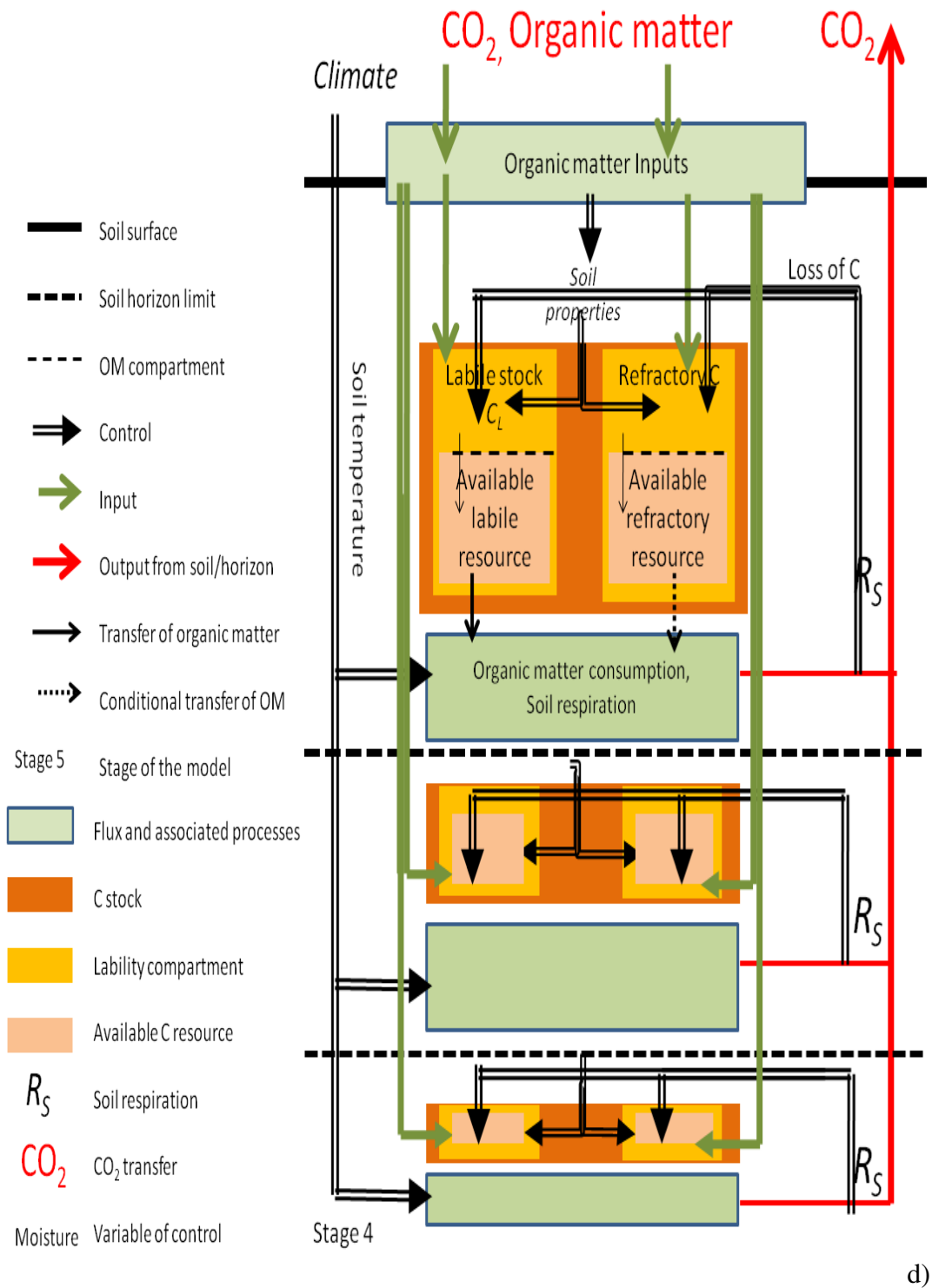
Figure 4.2 d: Stage 4 structure with several soil horizons; the inputs of CO 2 and organic matter going into the soil and ending up either in the labile or recalcitrant C compartment; the respiration rate is only function of the temperature and can use the stocks of labile and recalcitrant C; variables are explained in Appendix A4.1
