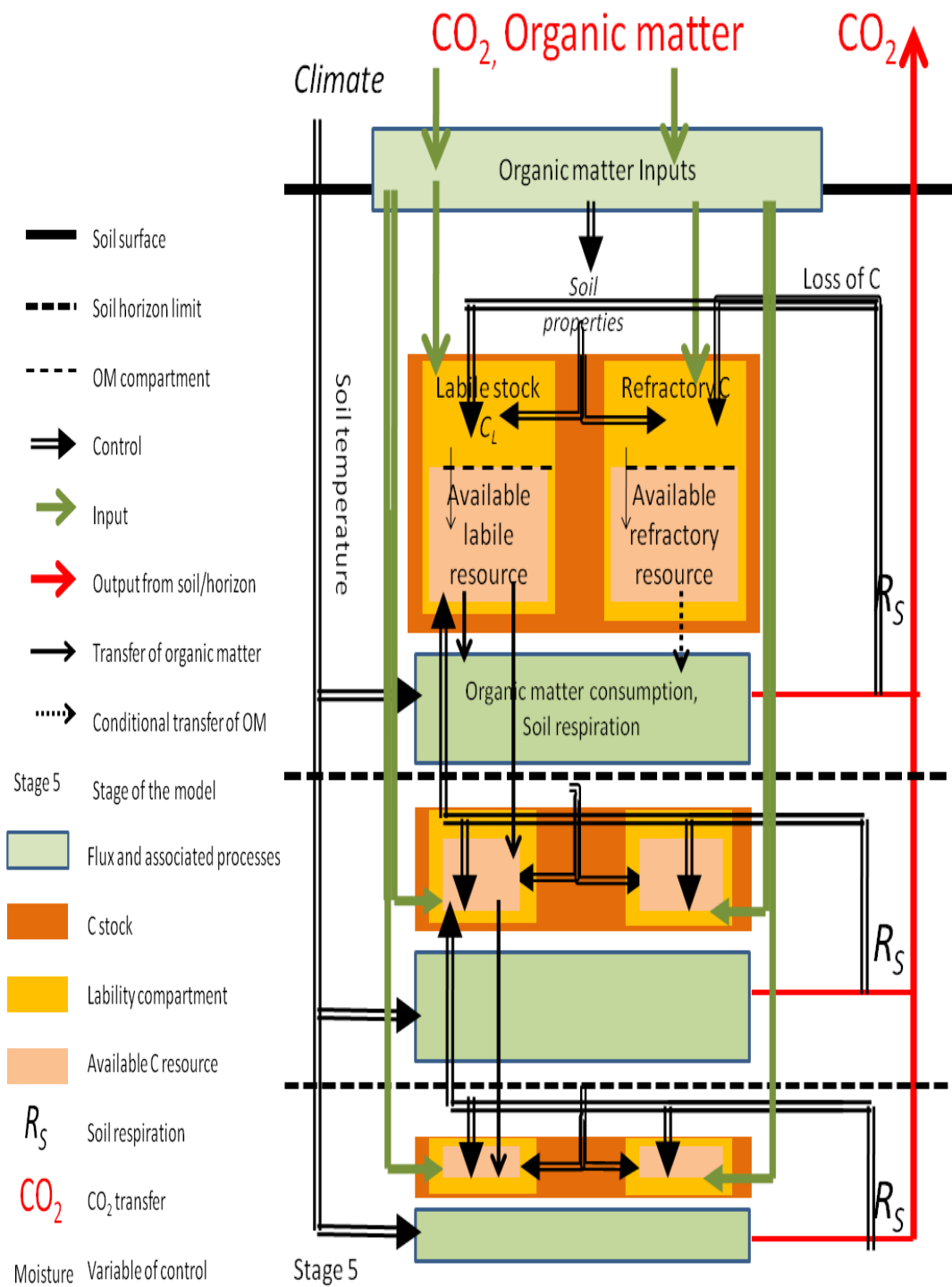
Figure 4.2 e: Stage 5 structure with several soil horizons; the inputs of CO 2 and organic matter going into the soil and ending up either in the labile or recalcitrant C compartment; the respiration rate are function of the temperature and can only use the existing soil C stocks; variables are explained in Appendix A4.1
