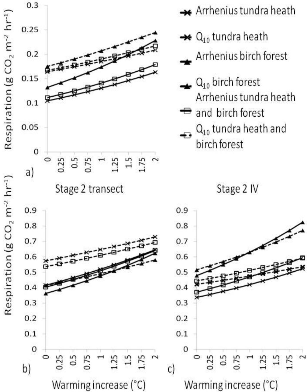
Figure 4.6: Annual average soil respiration (g CO 2 m -2 hr -1 ) simulated for increases in mean soil temperature from 0 to 2°C for tundra heath and birch forest soils (Stage 1 (a)) and using parameters from the transect profiles (Stage 2 (b)) and IV profiles parameters (Stages 2 (c))
