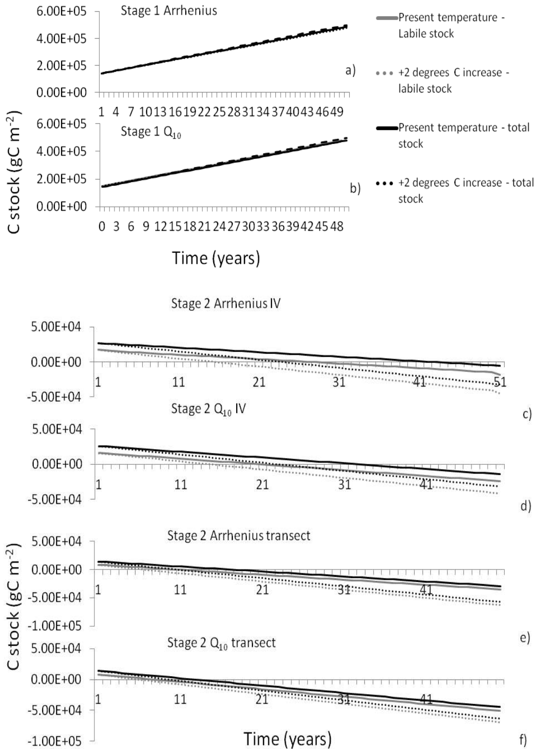
Figure 4.9: Labile and total C stocks depletion over 50 years with respiration calculated with the Arrhenius (Eq. 1) and Q_{10} (Eq. 2) equations for mean annual temperature increases of 0^\circ\text{C} and 2^\circ\text{C} ; for the tundra heath and birch forest landscapes (Stage 1, a and b), using parameters from the IV profiles (Stage 2, c and d) and transect profiles (Stage 2, e and f)
