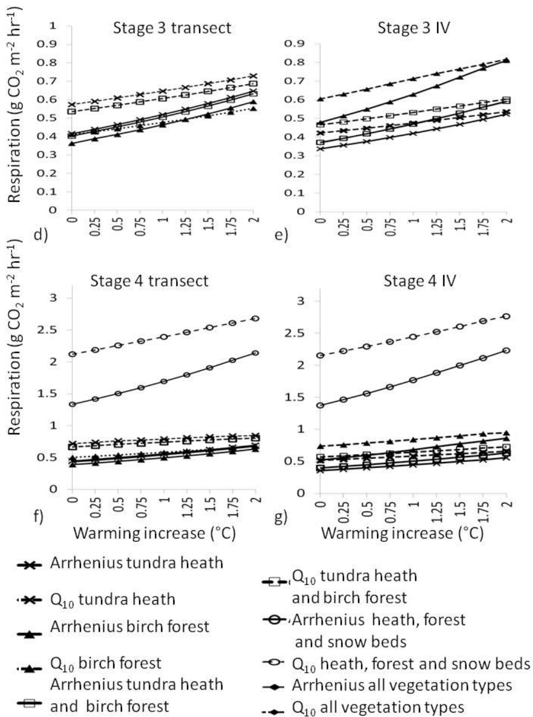
Figure 4.6: Annual average soil respiration (g CO 2 m -2 hr -1 ) simulated for increases in mean soil temperature from 0 to 2°C for tundra heath, birch forest and snow beds soils using parameters from the transect profiles (Stages 3 (d), 4 (f)) and IV profiles parameters (Stages 3 (e), 4 (g))
