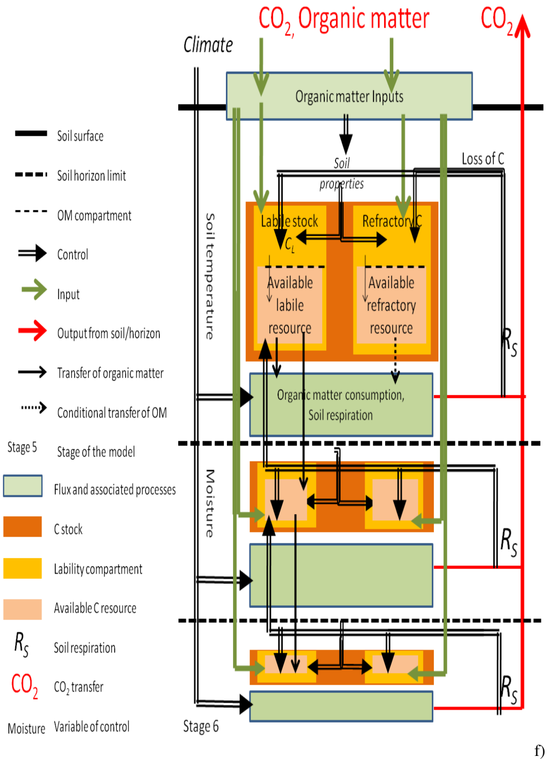
Figure 4.2 f: Stage 6 structure with several soil horizons; the inputs of CO 2 and organic matter going into the soil and ending up either in the labile or recalcitrant C compartment; the respiration rate is function of the temperature and the moisture; variables are explained in Appendix A4.1
