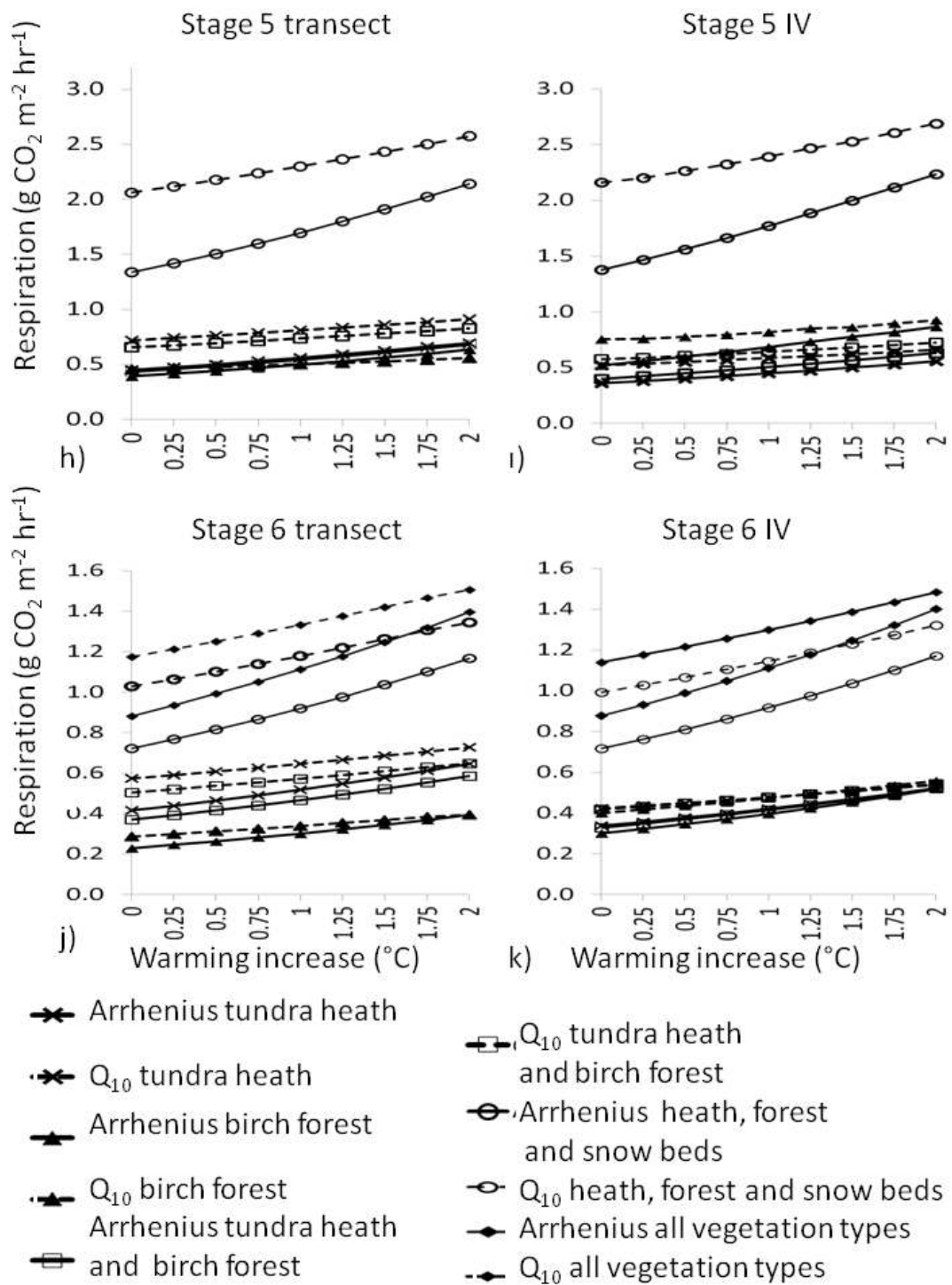
Figure 4.6: Annual average soil respiration (g CO 2 m -2 hr -1 ) simulated for increases in mean soil temperature from 0 to 2°C for birch forest, tundra heath, snow beds, Exposed heath and Sedge and wetlands soils, using parameters from the transect profiles (Stages 5 (h), 6 (j)) and IV profiles parameters (Stages 5 (i), 6 (k))
