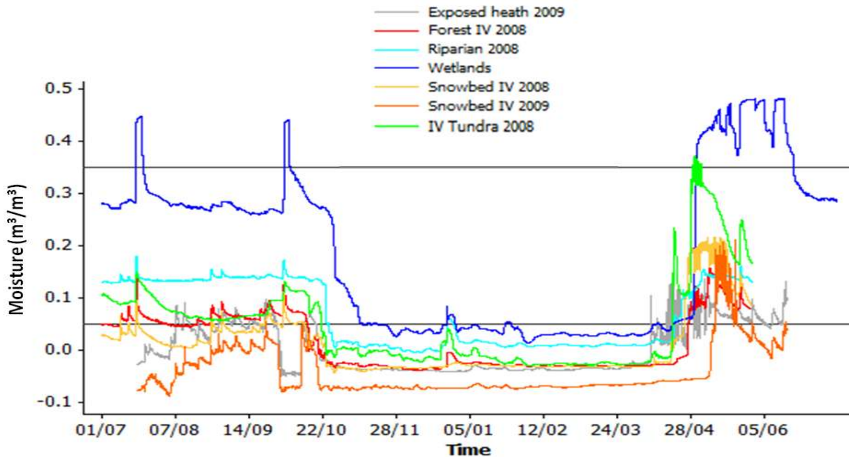
Figure 4.5: Moisture series ( m^3/m^3 ) in the Intensive Valley for soils under different vegetation categories, with reference lines for the 0.05 m^3/m^3 and 0.35 m^3/m^3 thresholds
