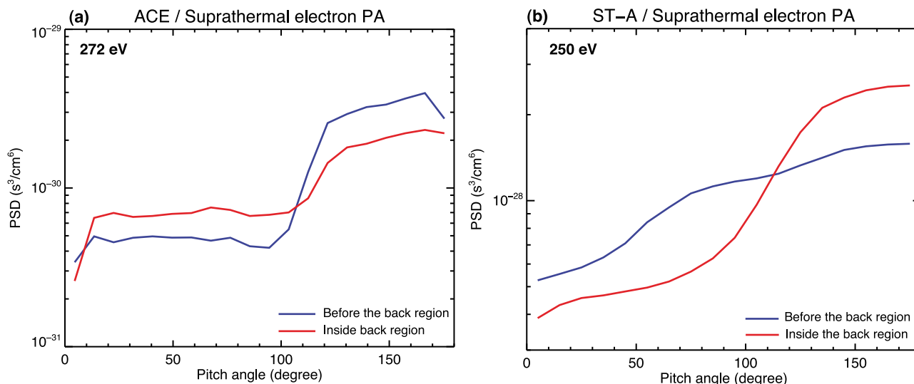
Figure 9. (a) ACE and (b) ST-A suprathermal electron pitch angle distributions obtained in the MC back region (red curve) and the MC core (blue curve), at times close to the boundary separating those two regions (see section 4.4 for details). Each is an average of consecutive PAD samples over 5 min.
