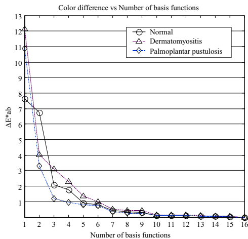
Figure 5 CIE color difference between the colors reproduced by the original 16-band multispectral image and K ( K = 1 \dots 16 ) basis functions derived from normal skin—for normal, dermatomyositis and palmoplantar pustulosis cases.
