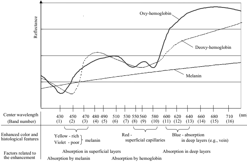
Figure 7 The wavelength and enhanced features. The horizontal axis represents the center wavelength of each band of MSC [(1)–(16)]. The plots are the spectral reflectance of melanin and hemoglobin media calculated from the absorption coefficients of the dyes. Since the short wavelength light does not penetrate deeper due to the light scattering property inside the skin, the influence of absorption at superficial layers are dominant in short wavelength, while the influence of deep layers appear in long wavelength components. According to these considerations, the features visualized by enhancing certain wavelength regions are also depicted.
