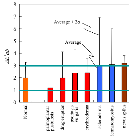
Figure 6 CIE color difference between the colors reproduced by the original 16-band multispectral image and three basis functions derived from normal skin. Bold bars represent the average and thin bars represent average + (standard deviation) \times 2 color differences of several areas selected from the images.
