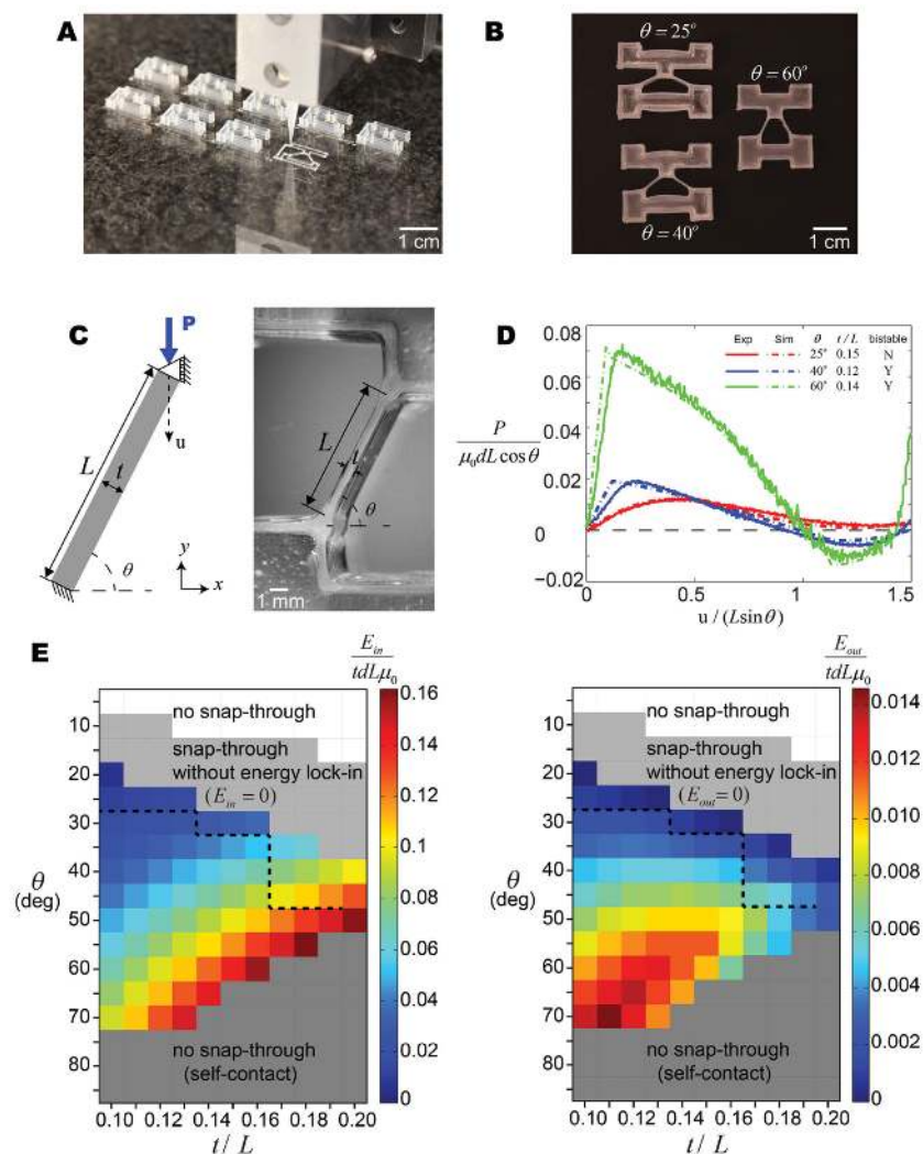
Figure 2. Mechanical response of a constrained, tilted elastic beam. a) Minimal functional structures, each with a unique combination of geometrical parameters, are rapidly printed (150–200 s each) using direct write 3D printing. b) Minimal structures consisting of two identical tilted beams. c) Schematic view showing the 2D model used in our FE simulations (left) and the corresponding beam in the fabricated minimal unit (right). d) Numerical and experimental force–displacement curves for three beams characterized by (\theta, t/L) = (25^\circ, 0.15) , (40^\circ, 0.12) , (60^\circ, 0.14) . The force is normalized by \mu_0 L d \cos \theta ( d denoting the out-of-plane thickness of the samples), while the displacement is normalized by L \sin \theta . e) Effect of \theta and t/L on the energy absorbed by the elastic beam ( E_{in} ) and the energy cost for the beam to snap back to its undeformed configuration ( E_{out} ). The black dashed lines indicate the experimentally observed transition between the geometries that result in bistability and those that merely possess the snap-through instability, but are not bistable.
