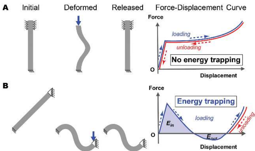
Figure 1. Energy absorption in an elastic beam. a) An elastic beam buckles when axially compressed, yet fully recovers to its initial shape when unloaded. b) A constrained tilted elastic beam may snap between two stable configurations, when one of its ends is moved vertically. In this case, the structure maintains its deformed shape when unloaded. Note: The bistable beams lock in most of the energy inserted into the system during loading ( E_{\text{locked}} = E_{\text{in}} - E_{\text{out}} ). Their initial (undeformed) configuration can be recovered when an amount of energy larger than E_{\text{out}} is supplied to the system.
