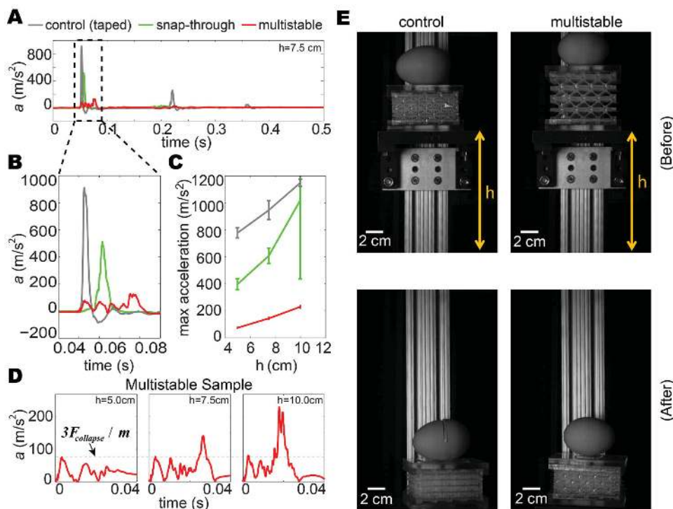
Figure 4. Drop tests. a) Acceleration–time curve for a multistable structure, the corresponding control sample (consisting of the same structures but taped to make all beams intentionally collapsed prior to the drop test), and a structure designed to possess snap-through instabilities but not energy-trapping, with samples dropped from h = 7.5 cm. b) Zoom-in of the acceleration–time curves. c) Peak acceleration amplitude as a function of the dropping height h for the multistable structure, the control sample, and the snap-through sample. The error bars indicate standard deviations from multiple ( N > 5 ) measurements. d) Acceleration–time curves for the multistable sample obtained from drop heights of h = 5, 7.5, and 10 cm. The horizontal dotted line indicates the collapse force divided by the mass of the egg for a line of tilted beams. The force is three times larger than that measured in the static compression tests since here we used three identical structures arranged in parallel for the drop tests. e) Drop of multistable and control samples with raw eggs attached to their top from h = 12.5 cm. The eggs attached to the multistable structures survive, while those on the control samples break upon impact.
