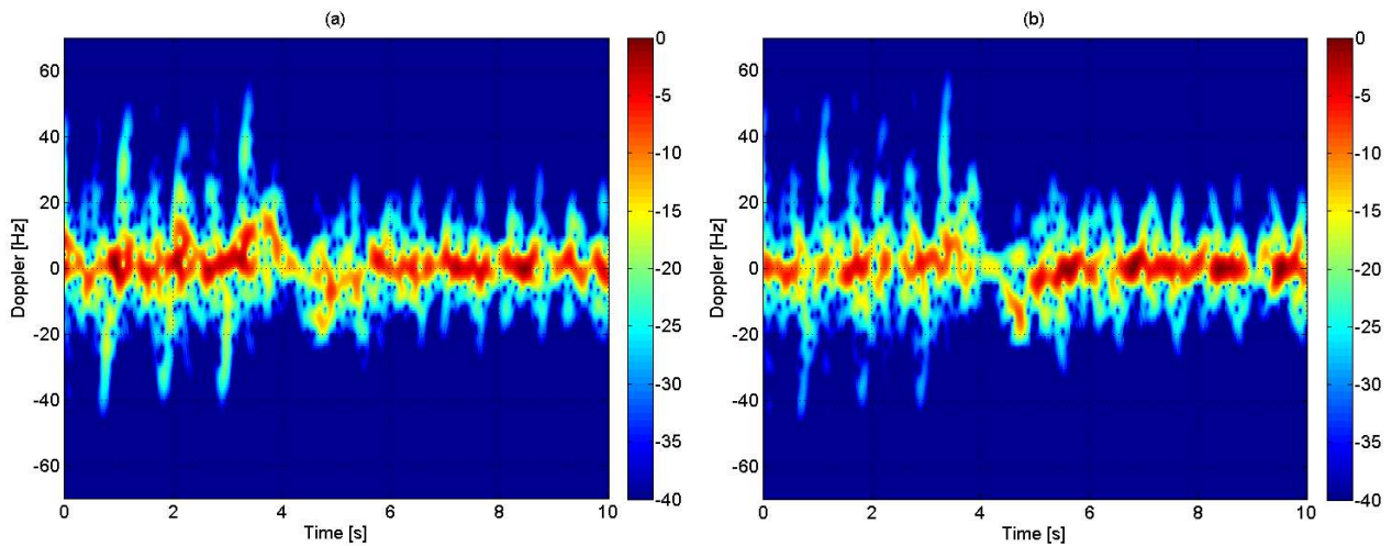
Figure 5 Micro-Doppler signature of a person walking on the spot empty-handed, picking up a metallic pole, and walking with the pole in both hands. Data from the monostatic (a) and one of the bistatic nodes (b)
