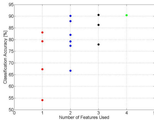
Figure 8 Classification accuracy for all possible combinations of feature vectors as input to the diagonal-linear classifier
