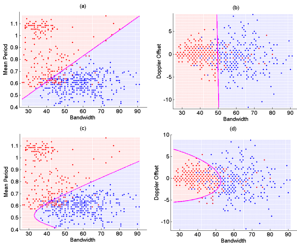
Figure 7 Examples of classifier plots for walking and walking with rifle data: (a) Linear classifier using bandwidth vs period (b) Bandwidth vs Doppler offset (c) Quadratic classifier using bandwidth vs period (d) Bandwidth vs Doppler offset
