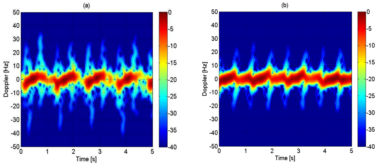
Figure 3 Micro-Doppler signature of a person walking on the spot (a), and walking on the spot without moving arms (b) – Data received at node 3
