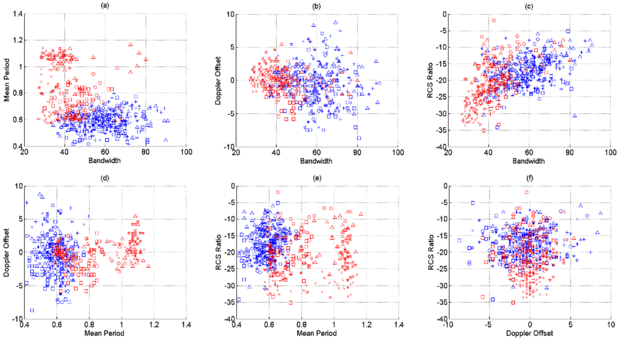
Figure 6 2D plots of samples extracted from walking and walking with rifle data for different combinations of features: (a) Bandwidth vs period, (b) Bandwidth vs Doppler offset (c) Bandwidth vs RCS Ratio (d) Period vs Doppler offset (e) Period vs RCS Ratio (f) Doppler offset vs RCS Ratio
