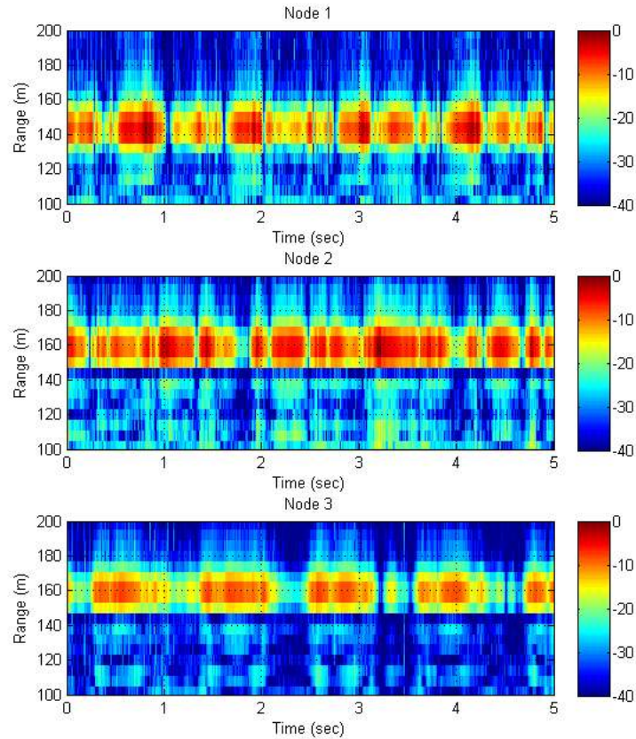
Figure 2 Range Time Interval (RTI) plots of human walking on the spot from Nodes 1, 2 and 3
