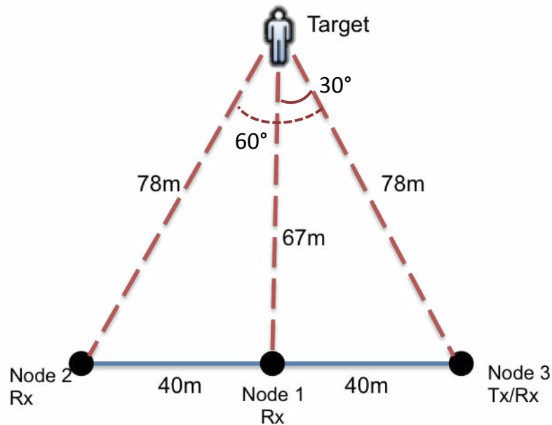
Figure 1 Model of the experimental geometry
