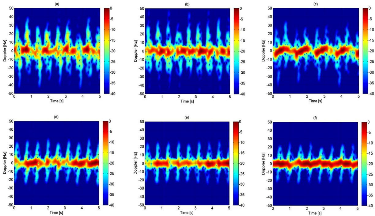
Figure 4 Micro-Doppler signature of a person walking on the spot with data received at node 1 (a), node 2 (b), and node 3 (c), and signature of a person walking on the spot while carrying a metal pole with both hands with data received at node 1 (d), node 2 (e), and node 3 (f)
