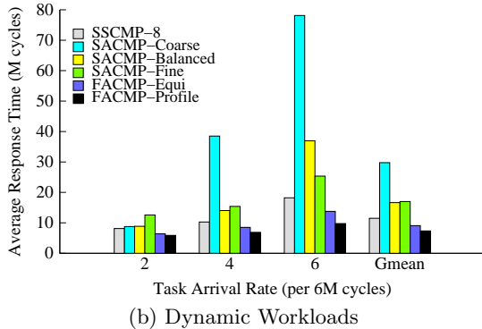
Figure 5: Adapting to task type.
