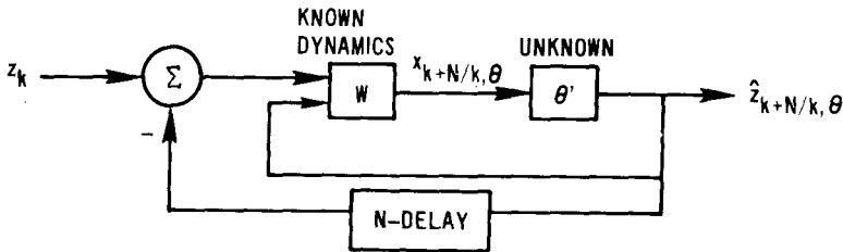
Fig. 4.4. N -step-ahead predictor conditioned on \theta .
