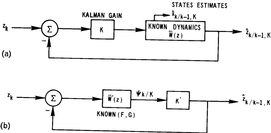
Fig. 4.1. Alternative structures of the Kalman one-step-ahead predictor.
