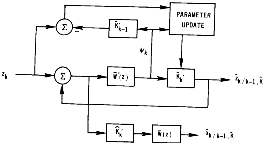
Fig. 4.2. Adaptive one-step-ahead predictor.
