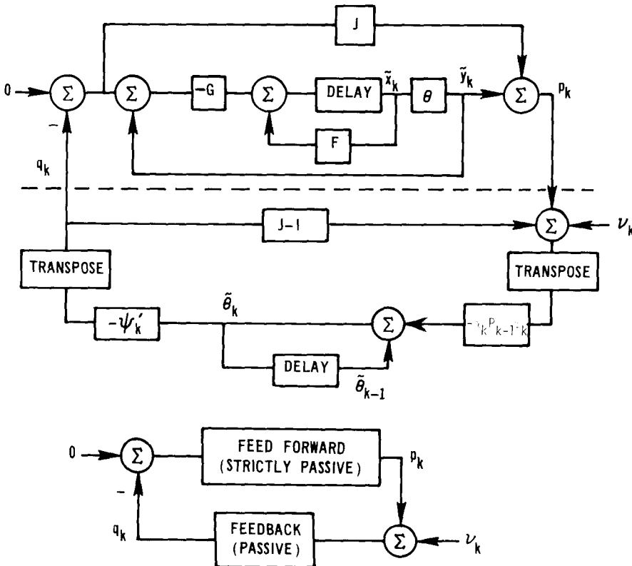
Fig. 3.1. Estimation error equations as two passive systems back to back.
