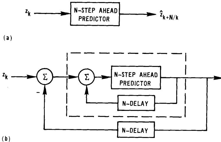
Fig. 4.3. Predictor re-organized as a feedback structure.
