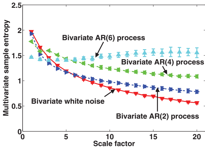
FIG. 5. (Color online) Multivariate multiscale entropy (MMSE) analysis for bivariate white noise and bivariate AR processes, each with 10 000 data points. The curves represent an average of 20 independent realizations and error bars the standard deviation (SD).
