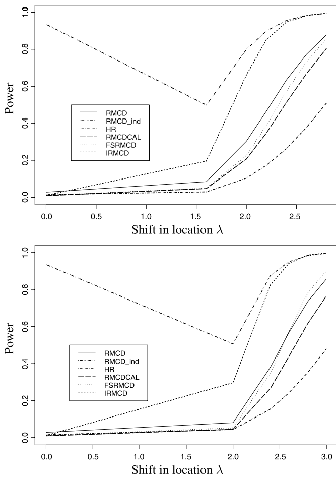
Figure 2. Power of MCD-based tests under a multivariate location-shift contamination model, for n = 200 and v = 5 . The nominal size for testing the simultaneous hypothesis (9) is \gamma = 0.01 . Upper panel: \tau = 0.05 . Lower panel: \tau = 0.20 . The cardinality h of the MCD subset is given by (3). Power is estimated on 5000 simulations for each value of \tau and \lambda .
