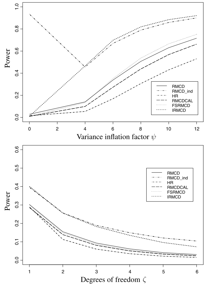
Figure 3. Power of MCD-based tests under alternative multivariate contamination models, for n = 200 , v = 5 , and \tau = 0.20 . The nominal size for testing the simultaneous hypothesis (9) is \gamma = 0.01 . Upper panel: radial contamination. Lower panel: multivariate t contamination. The cardinality h of the MCD subset is given by (3). Power is estimated on 5000 simulations for each value of \psi and \zeta .
