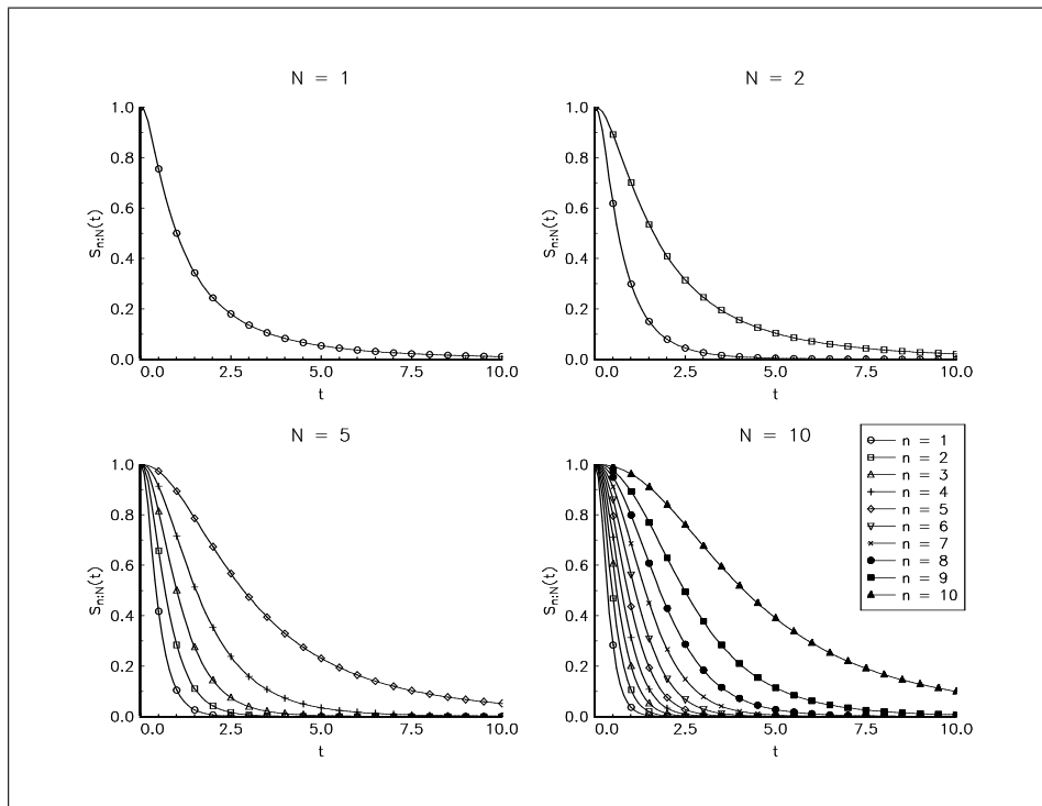
Figure 9: Survival function of order statistics T_{n:N}
