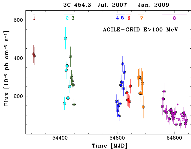
Figure 11. AGILE/GRID light curve at \approx 3 day resolution for E > 100 MeV in units of 10^{-8} photons \text{cm}^{-2} \text{s}^{-1} . Different colors correspond to different observing campaigns, as described in Table 1.
