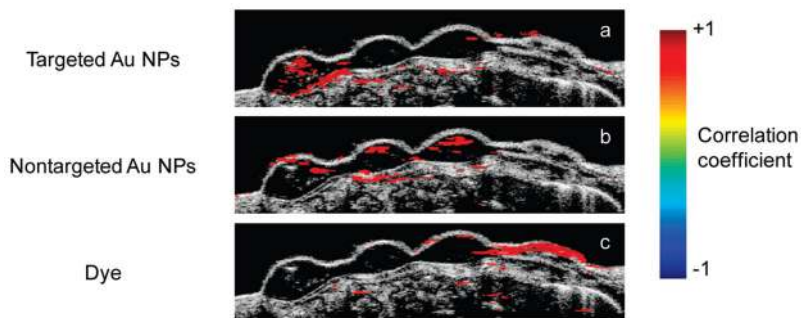
Figure 6. Correlation coefficient images overlaid on ultrasound image of the subcutaneous gelatin implants in mouse tissue ex-vivo . The correlation coefficient images were obtained by comparing multiwavelength photoacoustic images with optical spectra of (a) targeted Au NPs, (b) nontargeted Au NPs and (c) ADS740WS dye. Only correlation coefficient values greater than 0.75 are displayed in the images. The images measure 44 mm laterally and 9.1 mm axially.
