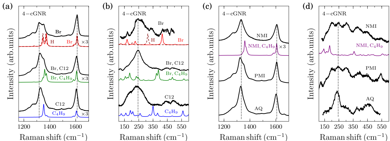
FIG. 3. (a) Optical and (b) acoustic region of the Raman spectra for 4-cGNRs with different edge functionalizations. Black (color) lines represent measured (calculated) spectra. In the simulated spectra, the G peak intensity has been rescaled ( \times 3 ), compared to the D peak, for clarity.
