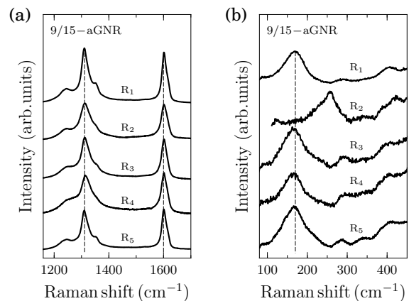
FIG. 6. (a) Optical and (b) acoustic region of the Raman spectra for 9/15-aGNRs with different edge functionalizations. The spectra are taken at 638\text{ nm} .
