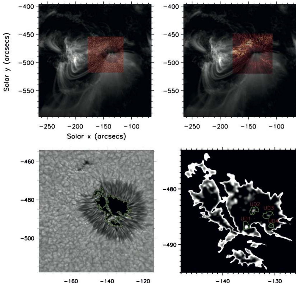
Fig. 14 The top panels display coronal EUV (171 Å) images taken by the AIA instrument onboard SDO on 2011 July 13 and interlaced with co-spatial and co-temporal ROSA 4170 Å continuum (upper left) and H \alpha (upper right) snapshots. It is clear the high degree of co-alignment precision now possible between multiwavelength and multi-instrument image sequences. The lower left panel shows the full ROSA 4170 Å continuum field-of-view, where solid green contours highlight the perimeter of the sunspot umbra. The lower right panel displays a magnification of the umbra itself, and reveals a number of small-scale intensity enhancements within the dark umbral background. Such umbral dots, labelled UD1, UD2, UD3 and UD4, display 3 minute oscillatory power several orders-of-magnitude higher than in the surrounding sunspot umbra (green contours) and are believed to be the locations where the intense coronal fans, each displaying prominent slow magnetoacoustic wave phenomena, are anchored. Images adapted from Jess et al. (2012a).
