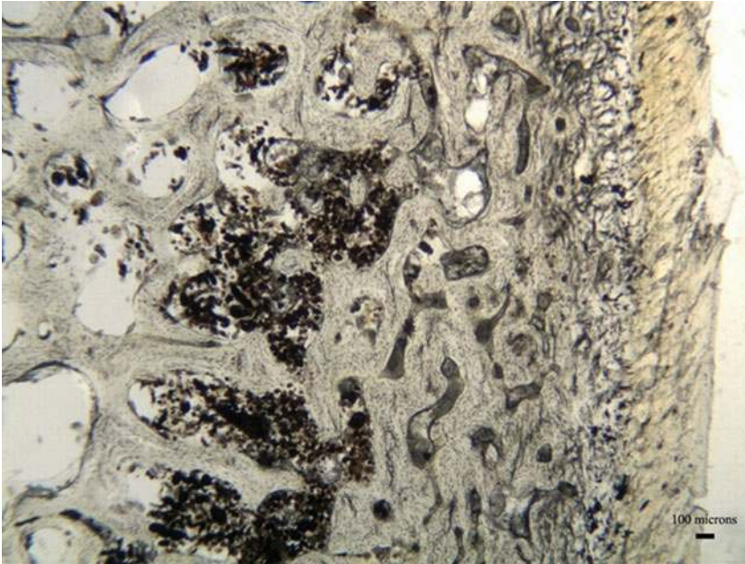
Figure 2. Micrograph of the patella thin section from a Yemeni mummy demonstrating immaculate histological preservation (soft tissue can be observed adhering to the periosteal surface to the right of the image).
