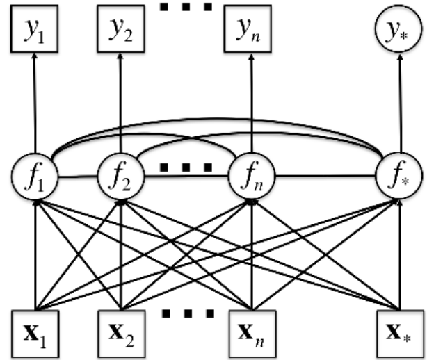
FIGURE 2. Graphical representation of observable x , y , (enclosed in squares), latent f , and unobservable y_* (enclosed in circles) variable relationships in Gaussian Process based regression task.
