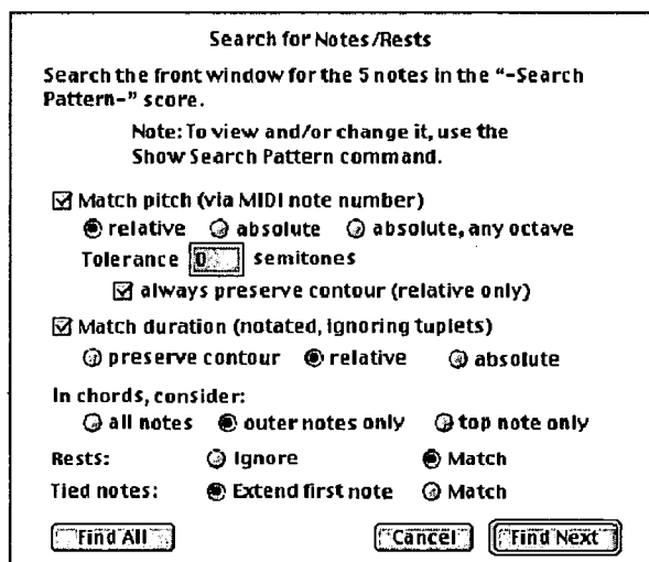
Fig. 4. Search Dialog
