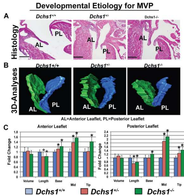
Figure 5. Developmental Etiology for MVP
