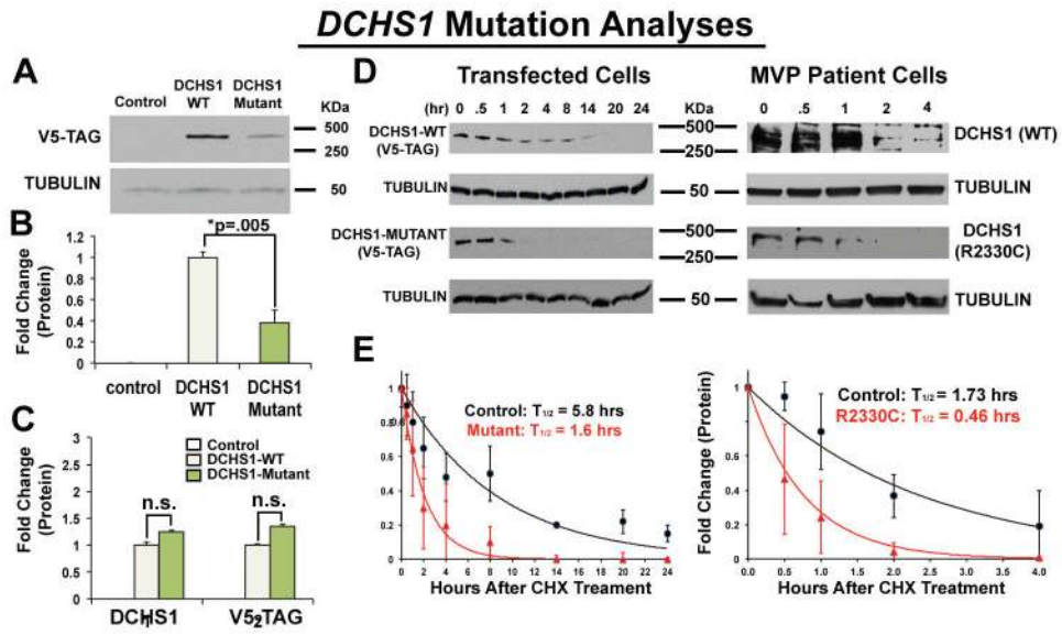
Figure 3. DCCHS1 Mutations Result In Diminished Protein Levels
