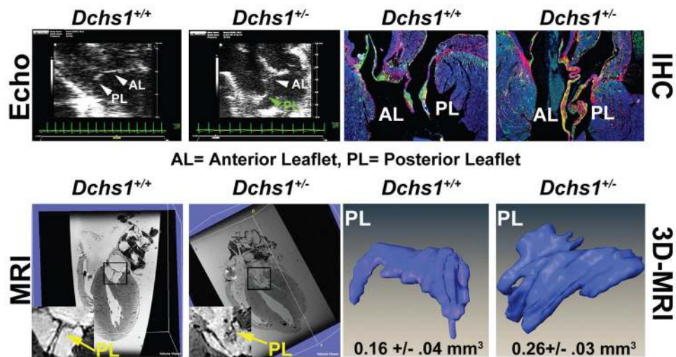
Figure 4. Dchs1 Deficiency Causes MVP and Myxomatous Degeneration in the Adult Mouse Echocardiography (Echo), MRI, Histopathology, and 3D reconstructions performed on 9-month old male Dchs1 +/+ and Dchs1 +/- mouse hearts. Echo: posterior leaflet prolapse in Dchs1 +/- (green arrow) (N=6/genotype). Immunohistochemistry (IHC): Dchs1 +/- (N=5) anterior, posterior leaflets (AL, PL) exhibit myxomatous degeneration and expansion of proteoglycan expression compared to Dchs1 +/+ (N=7), collagen (red), proteoglycans (green). MRI show posterior leaflet (PL) thickening in Dchs1 +/- (arrow-inset) compared to control littermates. 3D reconstructions of MRI: Dchs1 +/- mice exhibit thickened and elongated leaflets compared to Dchs1 +/+ . (Two-tailed Student t-test was used to calculate p -values; p =.01, N=4/genotype).
