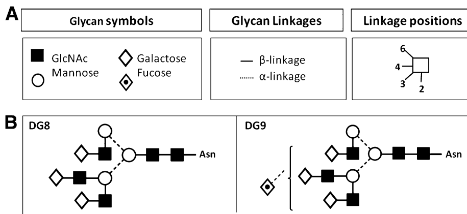
FIG. 1. A: Structural symbols for N -glycans, their linkages, and the abbreviations used. The Oxford nomenclature has been used to represent N -linked glycan composition and structure (20). B: Representations of the structures of the major glycans in DG8 and DG9 high-performance liquid chromatography peaks. Both are triantennary glycans. The only difference is the presence of a terminal fucose residue (◊) attached to one of the antennae of the glycans in DG9.
