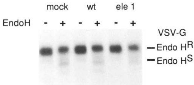
Figure 9. Dynamin mutants do not inhibit VSV-G transport between the ER and the Golgi stack. Vaccinia-infected cells were transfected with a plasmid containing the indicated dynamin construct and a plasmid encoding VSV-G protein (pAR-ts). Conversion of pulse-labeled VSV-G protein from an EndoH sensitive form found in the ER to an EndoH resistant form associated with the Golgi complex was determined as described in Materials and Methods.
