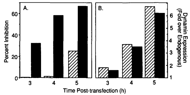
Figure 5. Time course of dynamain expression and inhibition of endocytosis. Vaccinia-virus infected HeLa cells were transfected with either wild-type dynamain (striped bars) or ele 1 GTP-binding domain mutant dynamain (solid bars), and incubated for the indicated times before harvesting. (A) Inhibition of Tfn endocytosis expressed relative to the level of endocytosis in mock-transfected cells at 3 h was determined as described in Materials and Methods. (B) Dynamain expression relative to endogenous levels was determined by Western blotting analysis as described in Materials and Methods.
