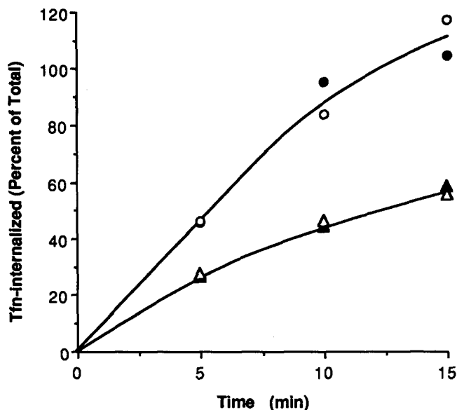
Figure 7. Expression of mutant dynamin blocks Tfn internalization at an intermediate stage in coated vesicle formation. Cells expressing either (○, ●) wild-type dynamin or ele I GTP-binding domain mutant dynamin (△, ▲) were harvested after an 8-h expression and incubated with BSST for the indicated times. The extent of Tfn internalization was assessed either by MesNa-resistance (●, ▲) or avidin accessibility (○, △) as described in Materials and Methods.
