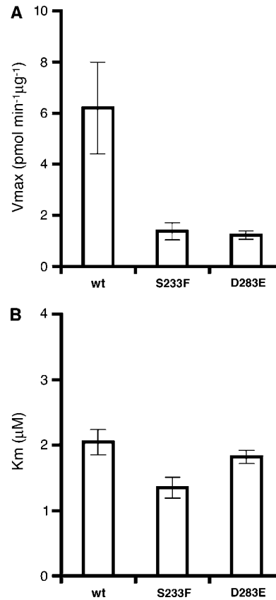
Figure 2. Hydrolysis rate ( V_{max} ) and affinity ( K_m ) of I-2N and its mutants for ATP. Purified I-2N and mutant forms of this protein (S233F and D283E) were incubated with different concentrations of [ \alpha^{32} P]ATP. Conversion of ATP to ADP was measured in an ATPase assay and quantified. The conversion rates at each ATP concentration were plotted in a Lineweaver-Burk graph and used to determine the V_{max} (pmol \text{min}^{-1} \mu\text{g}^{-1} ; A) and K_m ( \mu\text{M} ; B). All reactions were done at least in duplicate. The V_{max} and K_m value of I-2N presented is the mean based on the outcome with two independently purified protein preparations; error bars indicate the SD.
