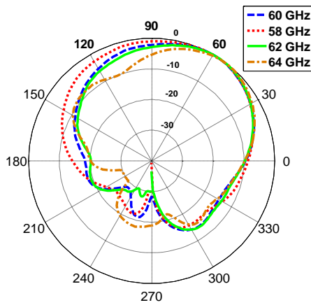
Fig. 10. The normalized radiation pattern of the DRA antenna with the metasurface consisting of 1x7 SSR array of unit cells at various frequencies in the H-plane (xz).
