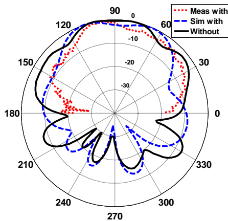
Fig. 12. The normalized simulated and measured radiation pattern of DRA antenna with and without metasurface consisting of a 1x7 array of SRR unit-cells at 60 GHz in the E-plane (yz).
