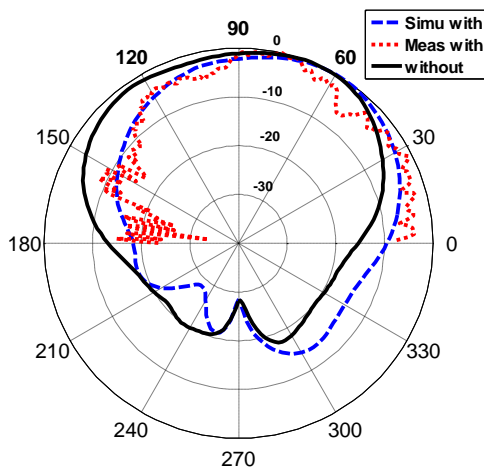
Fig. 11. The normalized radiation pattern of DRA antenna with and without metasurface consisting of 1x7 array of SRR unit-cells at 60 GHz in the H-plane (xz).
