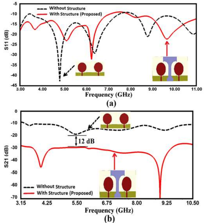
Fig. 3. The simulated scattering parameters of proposed UWB-MIMO antenna without (dashed line-black colour) and with decoupling structure (solid line-red colour). (a) Reflection coefficient ( S_{11} ) and (b) Transmission coefficient ( S_{21} ).
