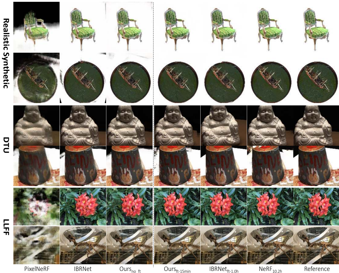
Figure 4. Rendering quality comparison. On the left, we show rendering results of our method and concurrent neural rendering methods [54, 46] by directly running the networks. We show our 15-min fine-tuning results and NeRF’s [34] 10.2h-optimization results on the right.
