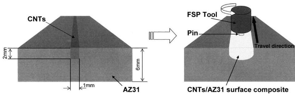
Fig. 2. Schematic of the friction stir processing.
