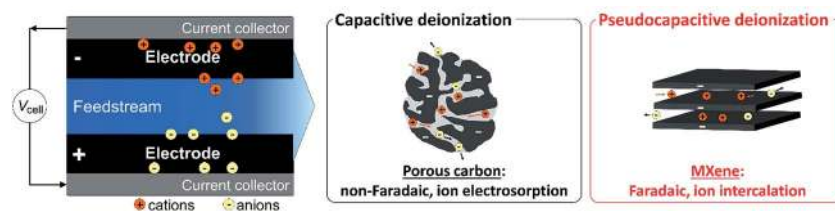
Fig. 4 Concept of electrochemical water desalination. Capacitive deionization accomplishes water desalination by non-faradaic (electrostatic) ion electrosorption at the surface of electrode materials. Pseudocapacitive deionization is accomplished by faradaic ion intercalation between the 2D-sheets of MXene. In both cases, anions and cations are removed.
