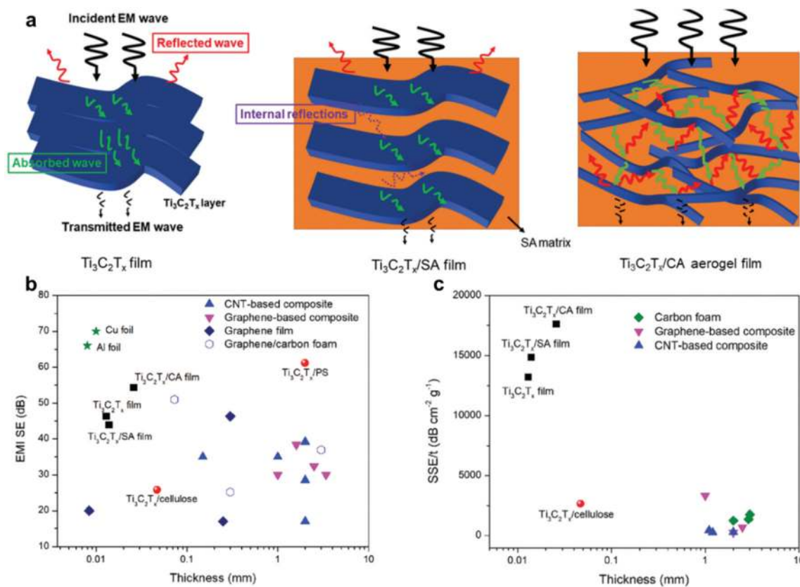
Fig. 15 (a) EMI shielding mechanism for freestanding Ti_3C_2T_x film, Ti_3C_2T_x /SA film, and Ti_3C_2T_x -CA aerogel. (b) Thickness-dependent EMI SE of various materials. (c) Different SSEA/t at different sample thicknesses. Reproduced with permission from ref. 47 (copyright 2019, Wiley-VCH).
