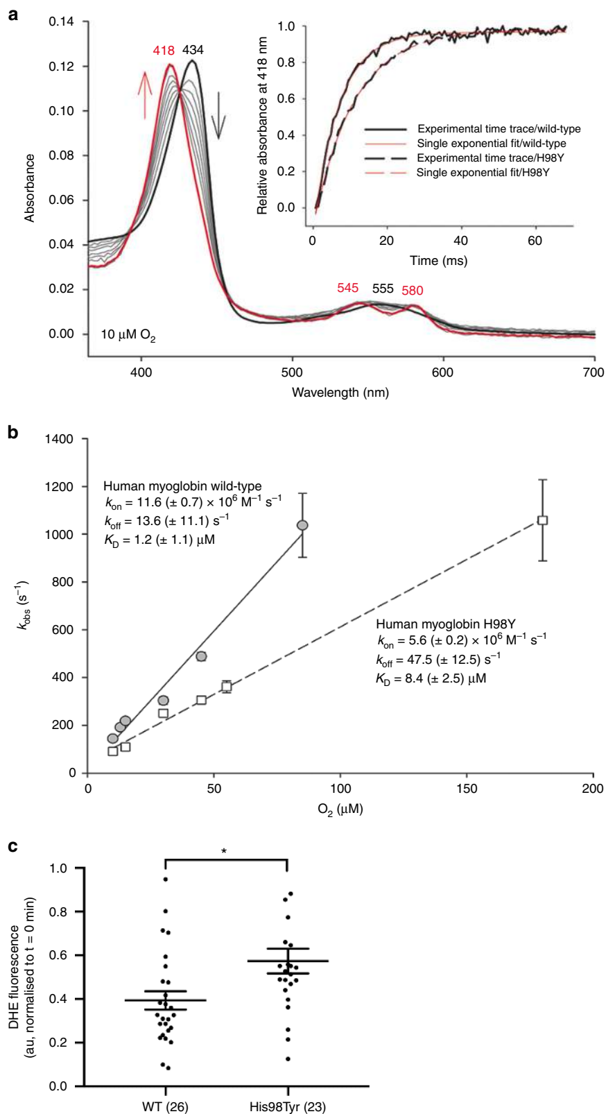
Fig. 7 Kinetics of dioxygen binding to wild-type human myoglobin and the variant His98Tyr. a Spectral changes upon reaction of 1 \mu\text{M} ferrous wild-type hMb (black line) with 10 \mu\text{M O}_2 . The final spectrum represents oxymyoglobin (red line, 68 ms after mixing). Gray lines represent spectra obtained at 0.68, 2.72, 4.08, 6.12, 8.84, 12.24, 34.00, and 51.00 ms after mixing. The inset depicts experimental time traces at 418 nm of wild-type hMb (solid black line) and p.His98Tyr MB (dashed black line) mixed with 10 \mu\text{M O}_2 and corresponding single-exponential fits (solid red line, wild-type MB; dashed red line, His98Tyr MB). b Linear dependence of k_{\text{obs}} values from the \text{O}_2 concentration for wild-type MM (gray circles, solid line) and p.His98Tyr MB (white squares, dashed line). c Basal intracellular superoxide levels in HEK293FT cells expressing WT or mutant MB-EGFP. Data presented as individual data points and the mean \pm SEM, numbers in parenthesis represent n . *indicates p = 0.007 (Mann-Whitney test, two-tailed)
