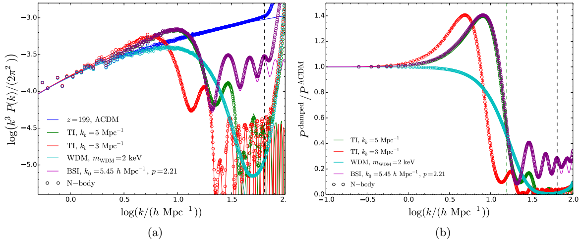
Figure 1. (a) Matter power spectra generated at z = 199 for different models as labelled. (b) Ratios of the linear damped power spectra relative to that from standard \Lambda CDM. Solid lines show the linear theory power spectra, while symbols represent the power spectra measured from the N-body ICs. The black vertical dashed line indicates the Nyquist frequency of the simulations. The green vertical dashed line in panel (b) shows the position of the half-mode wavenumber k_{1/2, \text{TI}5} for the thermal inflation matter power spectrum with k_b = 5 \text{ Mpc}^{-1} .
