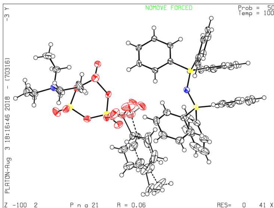
Figure S62: Single crystal X-ray Structure of [PPN][HNEt 3 ][1] with thermal ellipsoids set at 50%.
