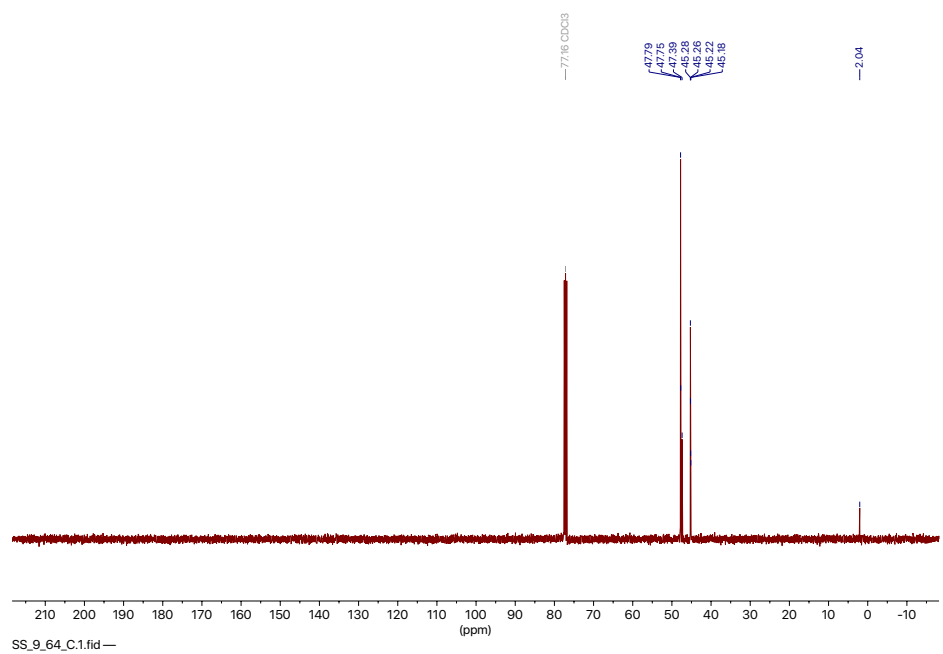
Figure S13: 13 C NMR spectrum of a mixture of 3 and 4 (chloroform- d , 100.6 MHz).
