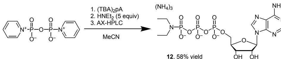
Figure S46: Synthesis of [\text{NH}_4]_3[\mathbf{12}] .
