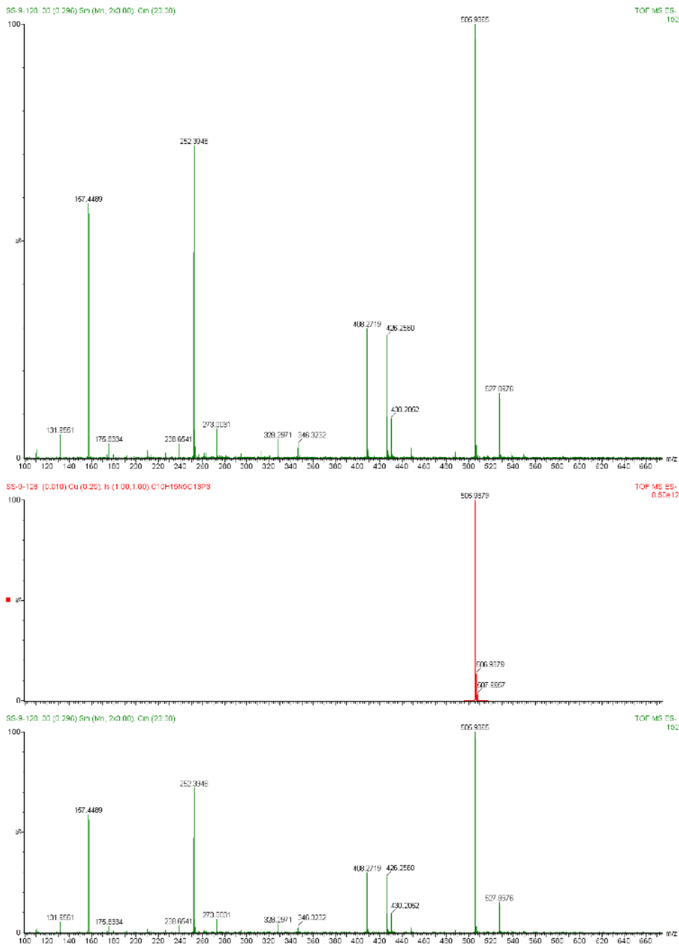
Figure S44: ESI-MS(-) of [NH_4]_4[11] ( H_2O/MeCN ) with zoomed in portion showing the molecular ion ( [C_{10}H_{14}N_5O_{13}P_3]H^- , bottom), and calculated isotope pattern (top).
