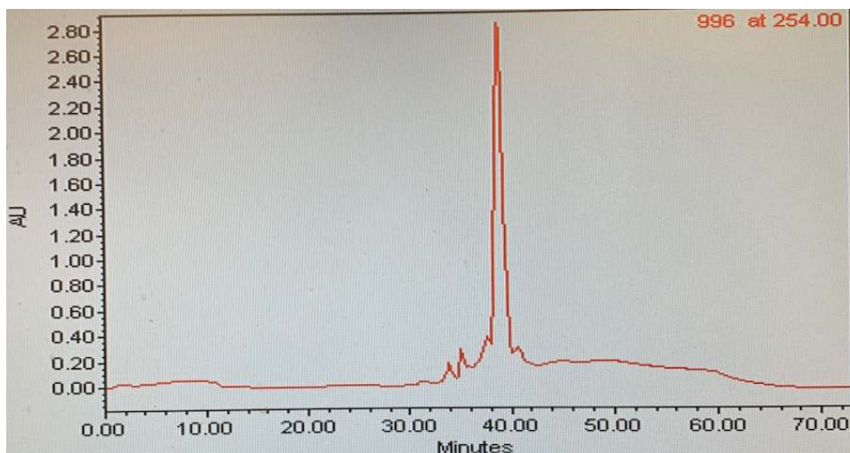
Figure S45: AX-HPLC trace of purified [\text{NH}_4]_4[\mathbf{11}] .
