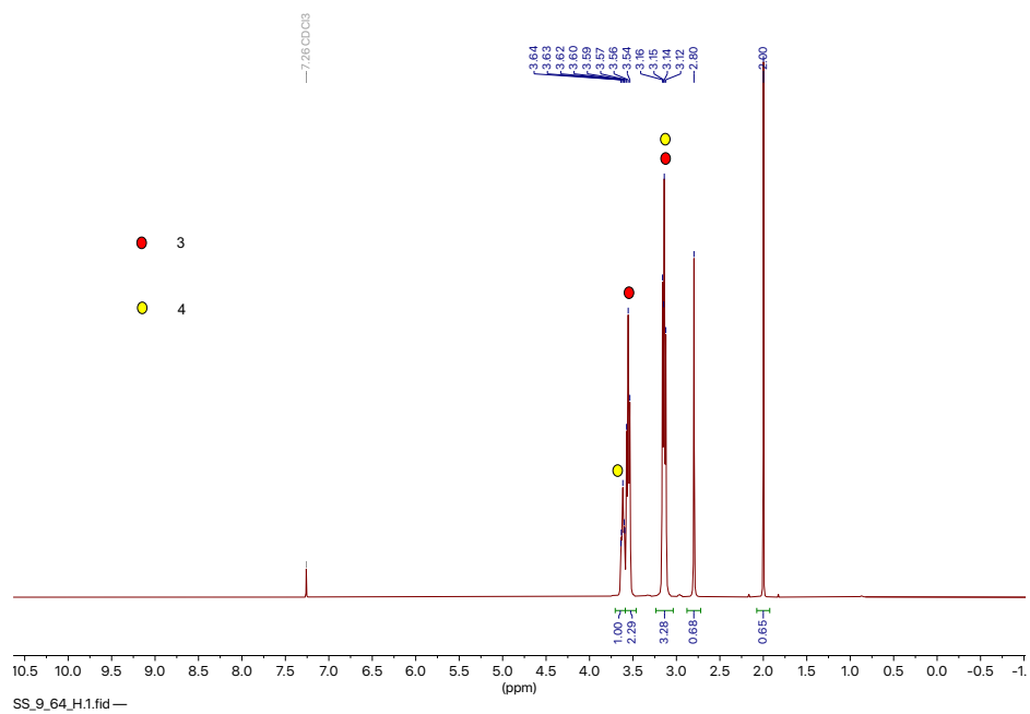
Figure S12: 1 H NMR spectrum of a mixture of 3 and 4 (chloroform- d , 400 MHz).
