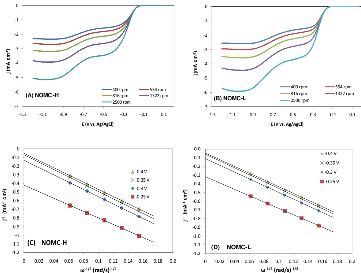
Figure 11. LSV curves for the NOMC electrocatalysts recorded in an O_2 -saturated 0.1 M KOH solution with a scan rate of 10 \text{ mV s}^{-1} at different rotation speeds (A and B), and the corresponding Koutěcký-Levich plots ( J^{-1} vs. \omega^{-1/2} ) at different electrode potentials for NOMC-H (C) and NOMC-L (D).
