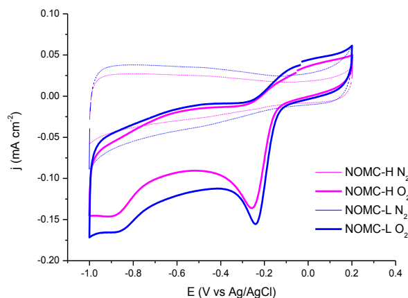
Figure 9. Cyclic voltammograms of NOMC-H and NOMC-L on a glassy-carbon RDE electrode in N_2 and O_2 -saturated 0.1 M KOH solution between 0.2 and -1.0 V at a scan rate of 50 \text{ mV s}^{-1} .
