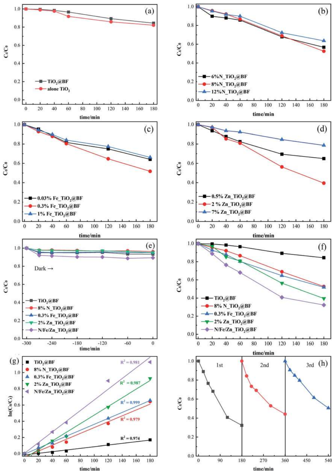
Fig. 7 (a) Photocatalytic activity of the same amount of TiO 2 without loading on BF and TiO 2 @BF, (b–d, f) photocatalytic activities (in the degradation of RhB) of TiO 2 @BF and G-TiO 2 @BF doped with different substances at different doping ratios, (e) dark adsorption curves, (g) photocatalytic degradation kinetics and (h) the stability and reusability tests of N/Fe/Zn-TiO 2 @BF for RhB removal.
