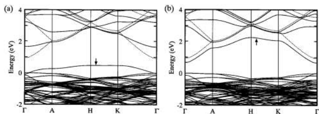
Fig. 12 Calculated band structure for ZnO supercells with (a) oxygen vacancy and (b) zinc interstitial. Note the direct competition of (a) p-type and (b) n-type conductivity between the two defect species. The valence band maximum is defined at zero energy. The highest occupied state is indicated by an arrow in each. Adapted with permission from Oba et al. 99 Copyright 2001 AIP Publishing LLC.
