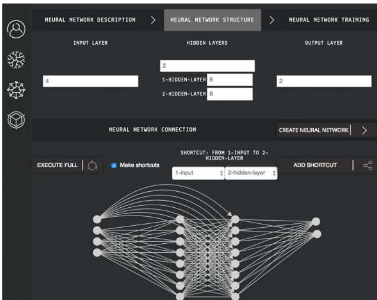
Fig. 6 The user specifies the neural network structure
