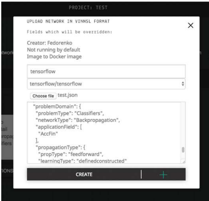
Fig. 5 The user uploads the neural network paradigm description in ViNNsL format
