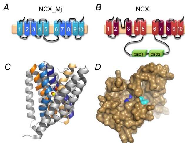
Figure 1. Molecular properties of the Na + /Ca 2+ exchanger
