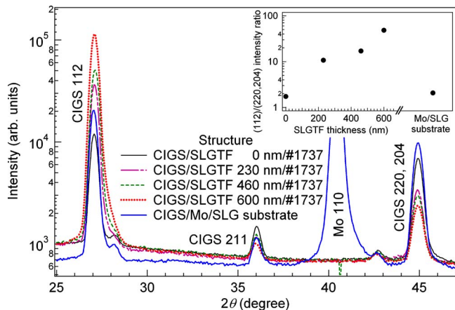
FIG. 4. (Color online) Variations in the XRD patterns of CIGS films with various SLGTF thicknesses. The XRD pattern of a CIGS film grown on a Mo/SLG substrate is shown for reference. The inset figure shows the (112)/(220, 204) intensity ratio of the XRD patterns.
