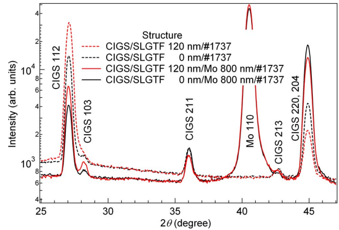
FIG. 5. (Color online) XRD patterns of CIGS films grown on #1737 substrates with and without SLGTF and Mo back contact layers.
