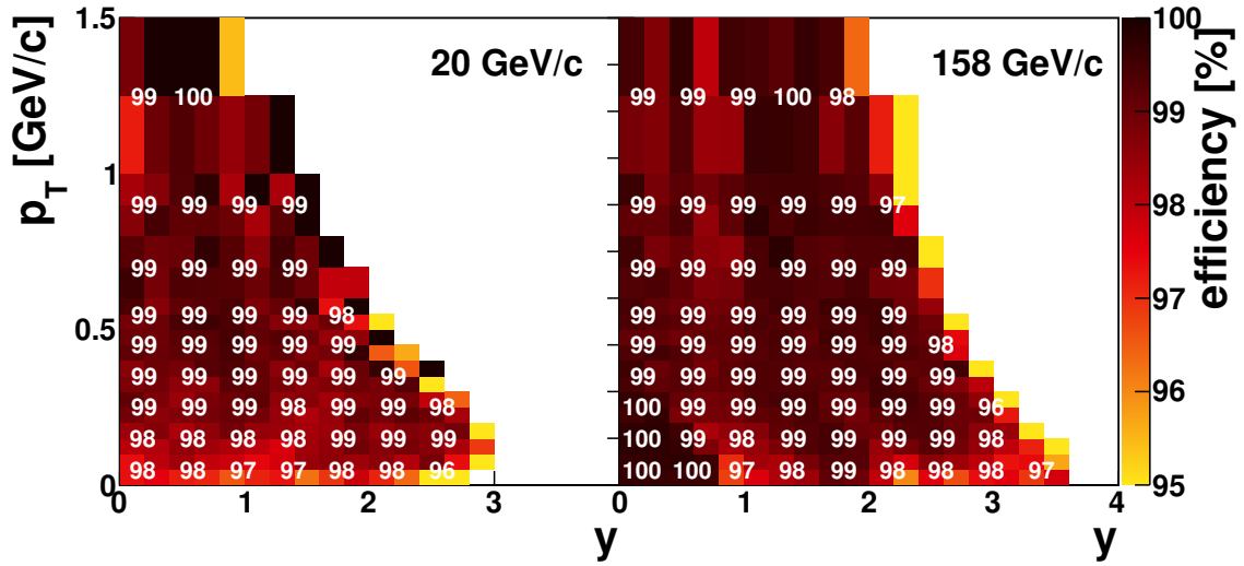
Figure 18. The reconstruction efficiency of negatively charged pions produced in p+p interactions at 20 ( left ) and 158 GeV/ c ( right ) as a function of pion rapidity and transverse momentum. The magnetic fields were set for a total bending power of 1.1 and 9 Tm at 20 and 158 GeV/ c , respectively.
