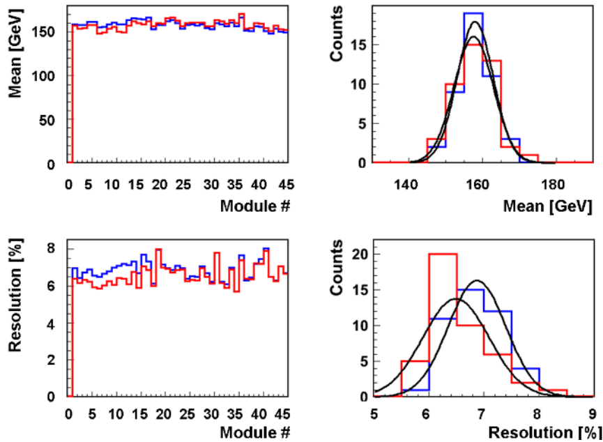
Figure 29. Mean values of reconstructed incident 158 GeV/ c proton energy in the PSD modules ( top left ) and distributions of mean values for the 44 modules ( top right ). Energy resolution for 158 GeV/ c protons ( bottom left ) and distributions of resolution for the 44 modules ( bottom right ).
