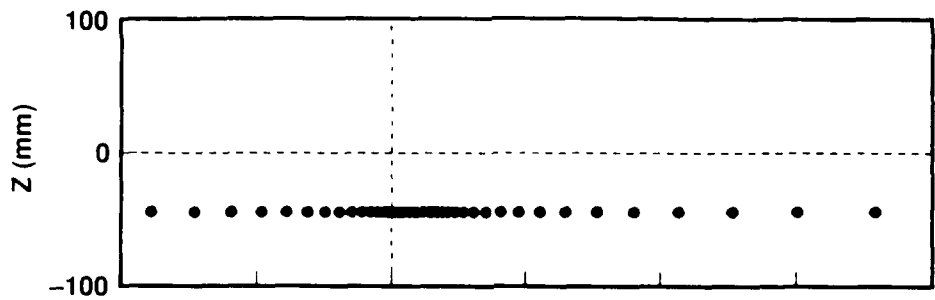
(a) Fine grid across vortex core
