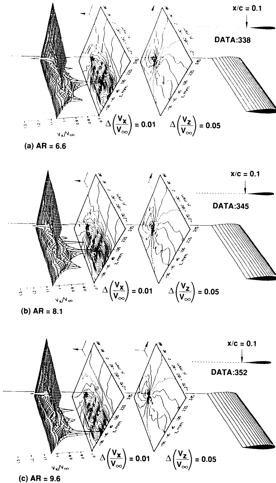
Figure 59. Vertical and streamwise velocity contours around trailing vortex from c = 30 cm wing (square tip) at x/c = 0.1 with Re = 1.5 \times 10^6 and \alpha = 12^\circ for different aspect ratios.
