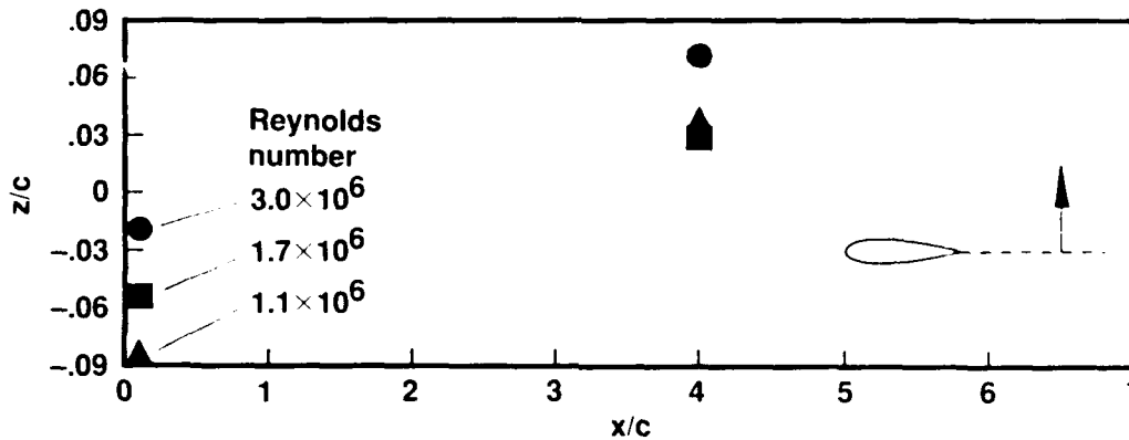
(c) Vertical displacement of vortex core (Referenced to trailing edge when \alpha = 0^\circ )
