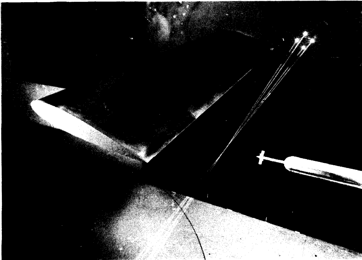
Figure 8. Vortex meter used to locate trailing-vortex core. (a) Cruciform and Hall-effect transducer elements of vortex meter. (b) Vortex meter positioned near wing tip.
