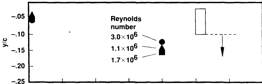
(b) Spanwise displacement of vortex core
