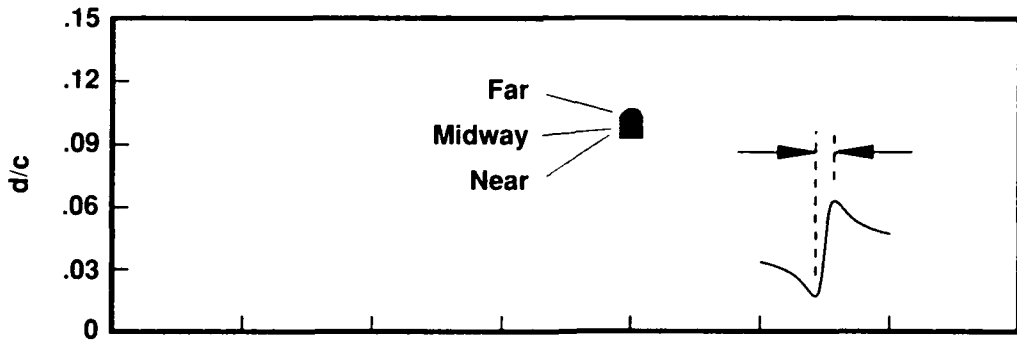
(a) Diameter of vortex core
