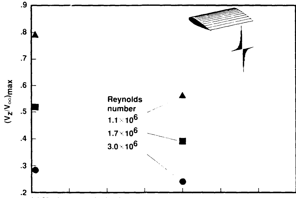
(a) Maximum vertical-velocity component
