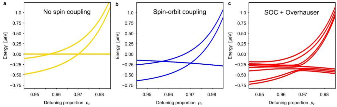
Extended Data Fig. 3 | Effects of spin-coupling mechanisms. Calculated spectra of the system in the region of \rho_\epsilon close to the level crossing of the s=1/2 and s=3/2 energies, comparing the effects of different mechanisms for spin coupling. a , Spectrum without any spin coupling effects. b , Spectrum including only spin-orbit coupling (SOC) effects. c , Sample spectrum with
