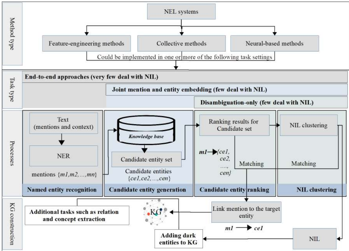
FIGURE 8. General NEL model along with central sub-tasks and techniques.
