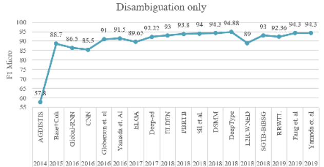
FIGURE 10. SOTA disambiguation-only results for NEL (AIDA-CoNLL).
