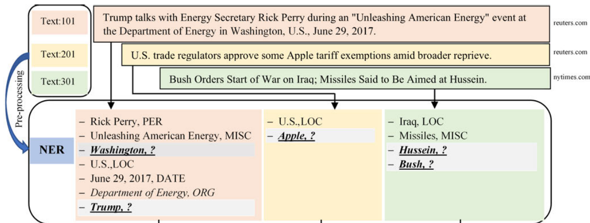
FIGURE 4. Example of a NER task.
