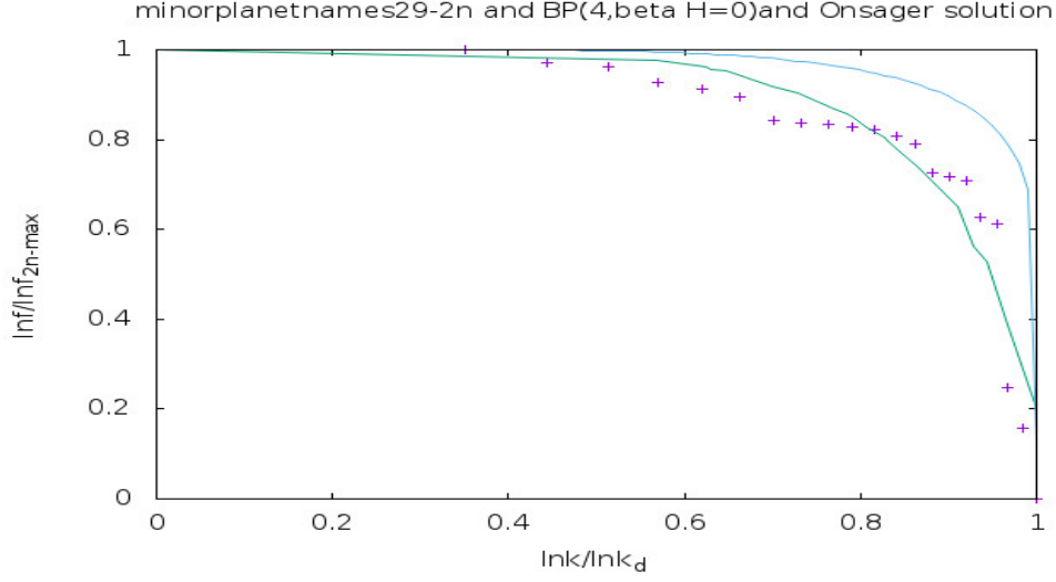
FIG. 19. Vertical axis is \frac{\ln f}{\ln f_{2n-max}} and horizontal axis is \frac{\ln k}{\ln k_{lim}} . The + points represent the names of the minor planets discovered up to 1929 end, with the fit curve being Bethe-Peierls curve in presence of four nearest neighbours and in absence of external magnetic field BP(4, \beta H = 0) . The uppermost curve is the Onsager solution.
