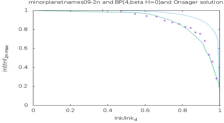
FIG. 11. Vertical axis is \frac{\ln f}{\ln f_{2n-max}} and horizontal axis is \frac{\ln k}{\ln k_{lim}} . The + points represent the names of the minor planets discovered up to 1909 end, with the fit curve being Bethe-Peierls curve in presence of four nearest neighbours and in absence of external magnetic field BP(4, \beta H = 0 ). The uppermost curve is the Onsager solution.
