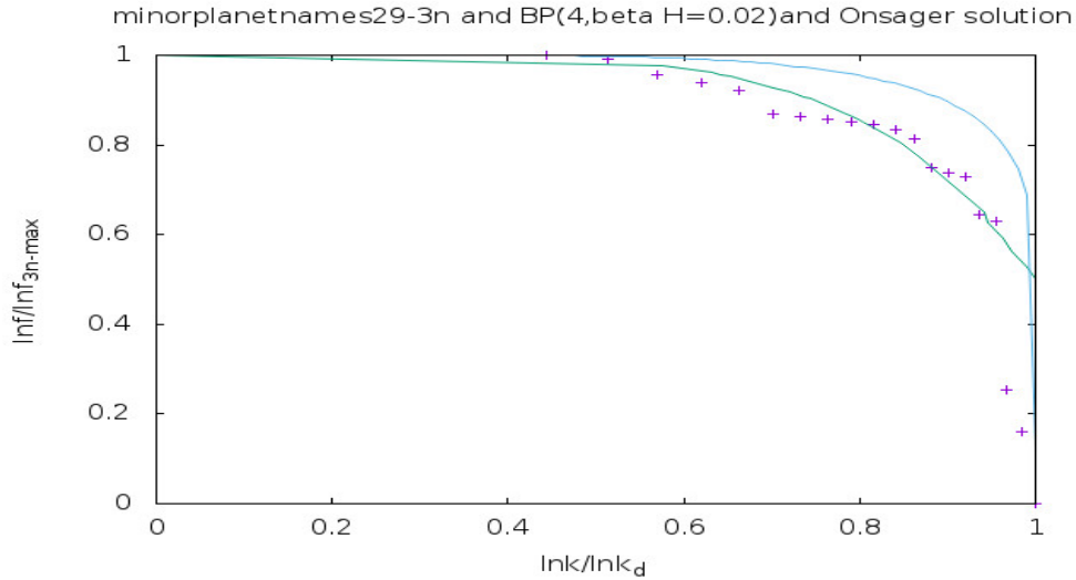
FIG. 20. Vertical axis is \frac{\ln f}{\ln f_{3n-max}} and horizontal axis is \frac{\ln k}{\ln k_{lim}} . The + points represent the names of the minor planets discovered up to 1929 end, with the fit curve being Bethe-Peierls curve, BP(4, \beta H = 0.02) , in presence of four nearest neighbours and little external magnetic field, m = 0.01 or, \beta H = 0.02 . The uppermost curve is the Onsager solution.
