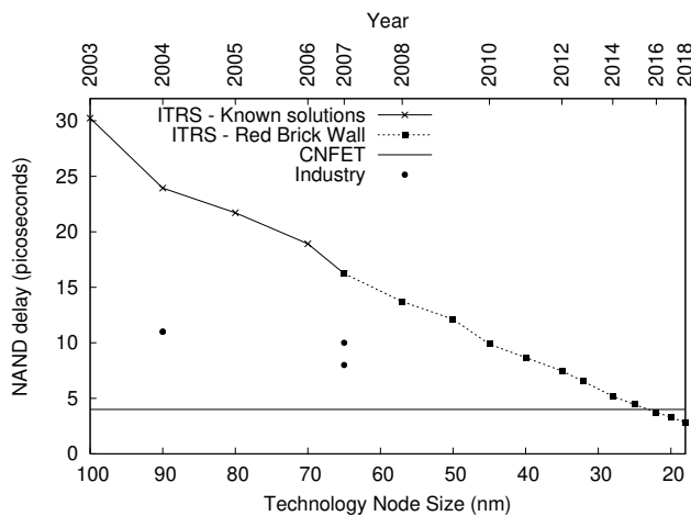
Figure 1. Nanoscale Device Performance
