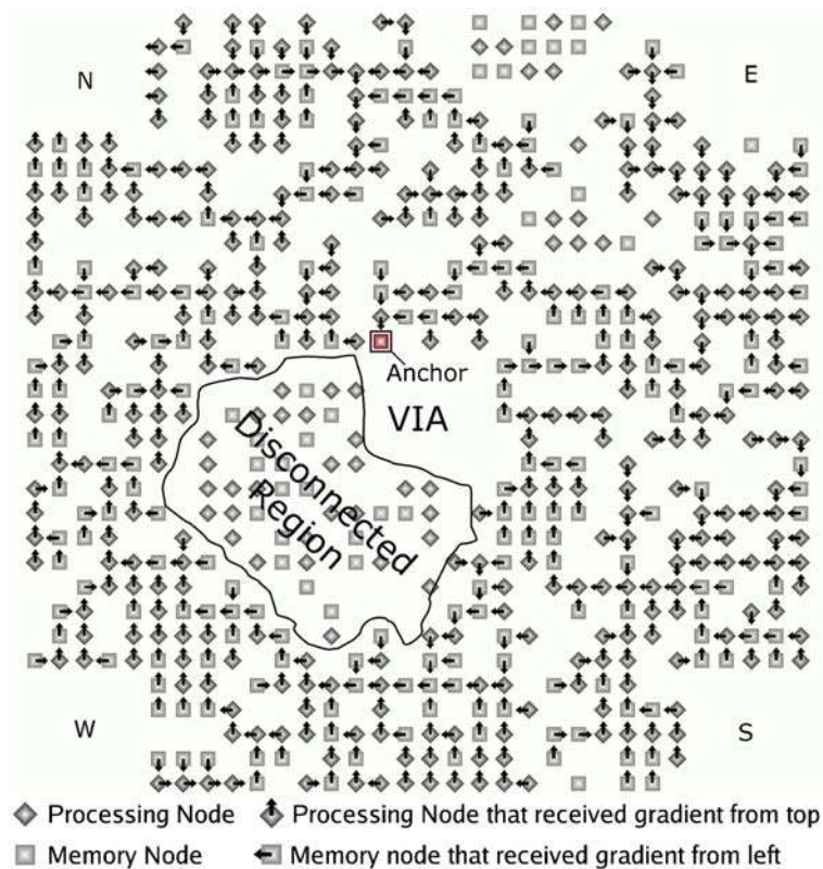
Figure 6. A 32 x 32 grid of memory and processing nodes with one established gradient (North)
