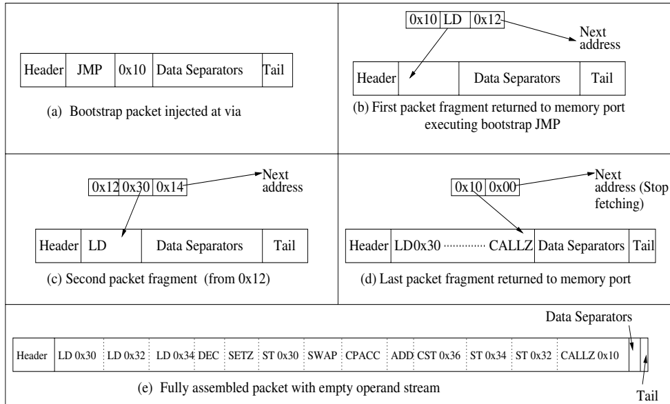
Figure 10. Bootstrapping the fibonacci execution packet with a JMP
