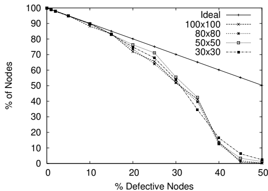
Figure 7. Percentage of nodes reachable by gradient broadcast for varying defect rates
