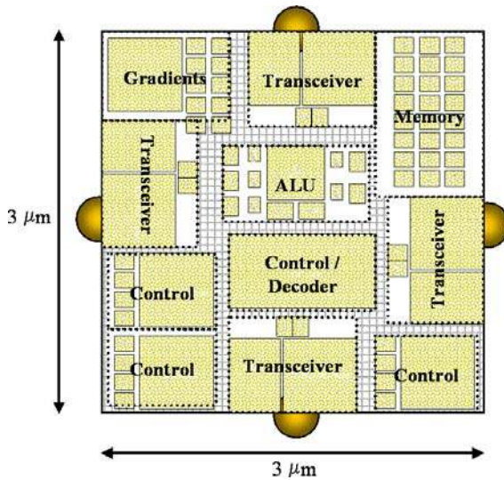
Figure 9. Node floorplan
