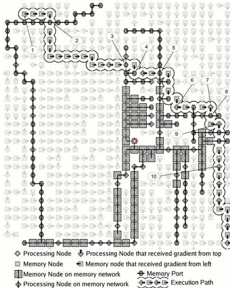
Figure 11. The path of Fibonacci code in one direction through configured network with 1024 nodes and 3% defects. Unused nodes in the execution network appear faded, defective nodes are omitted. 1: Bootstrap packet injected via, 2: JMP executes at port, 3: LD 0x30 executes at port, 4: LD0x32 executes at port, 5: LD 0x34 executes at port, 6: DEC at processing node, 7: CMPZ executes at processing nodes, 8: ST 0x30 executes at port, 9: SWAP executes at processing node, 10: ADD executes at processing node.
